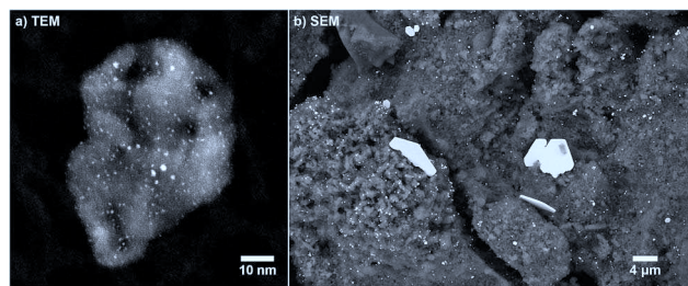
Fig. 3 (a) TEM image (STEM, 910k \times magnification) of a fresh Pt/Al 2 O 3 sample. (b) SEM image (BSE, 8k \times magnification) of a sample aged for 24 h at 950 °C.
