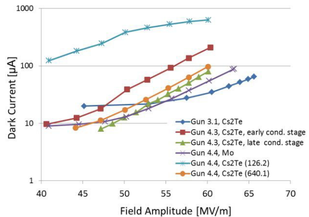
Figure 4: Comparison of the measured dark currents as a function of electric field amplitude.
