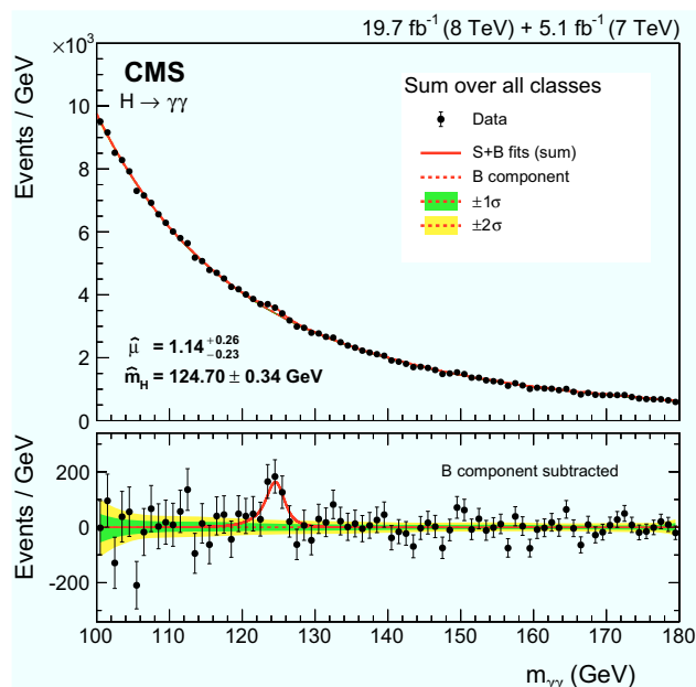
Fig. 17 Sum of the 25 signal-plus-background model fits to the event classes in both the 7 and 8 TeV datasets, together with the data binned as a function of m_{\gamma\gamma} . The 1\sigma and 2\sigma uncertainty bands shown for the background component of the fit are computed from the fit uncertainty in bins corresponding to those used to display the data. These bands do not contain the Poisson uncertainty that must be included when the full uncertainty in the number of background events in any given mass range is estimated. The lower plot shows the residual data after subtracting the fitted background component
