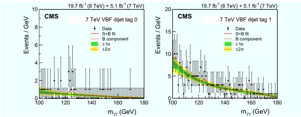
Fig. 11 Events in the two VBF dijet-tagged classes of the 7 TeV dataset, binned as a function of m_{\gamma\gamma} , together with the result of a fit of the signal-plus-background model. The 1\sigma and 2\sigma uncertainty bands shown for the background component of the fit include the
