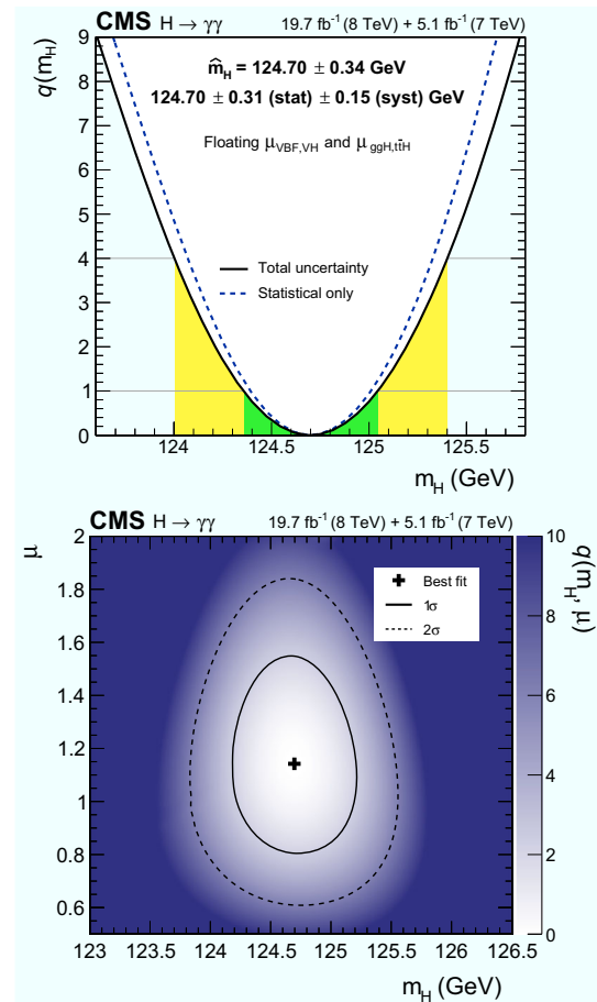
Fig. 22 (top) Scan of the likelihood ratio, q , as a function of the hypothesised mass when \mu_{ggH, t\bar{t}H} and \mu_{VBF, VH} are allowed to vary independently. (bottom) Map of q(m_H, \mu) showing the 1\sigma and 2\sigma regions, and the best-fit point (\hat{m}_H, \hat{\mu}) = (124.70 \text{ GeV}, 1.14)
