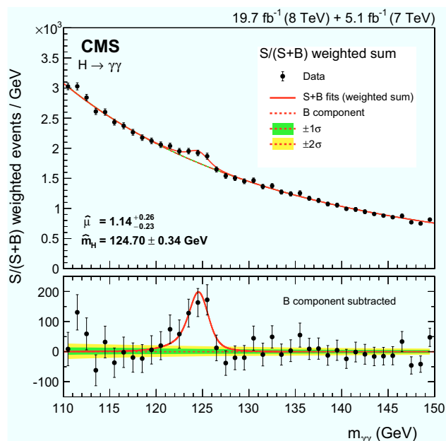
Fig. 19 Diphoton mass spectrum weighted by the ratio S/(S+B) in each event class, together with the background subtracted weighted mass spectrum
