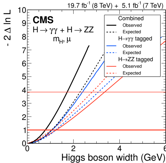
Figure 3: Likelihood scan as a function of the width of the boson. The continuous (dashed) lines show the observed (expected) results for the H \rightarrow \gamma\gamma analysis, the H \rightarrow ZZ \rightarrow 4\ell analysis, and their combination. The data are consistent with \Gamma_{\text{SM}} \sim 4 MeV and for the combination of the two channels the observed (expected) upper limit on the width at the 95% CL is 1.7 (2.3) GeV.
