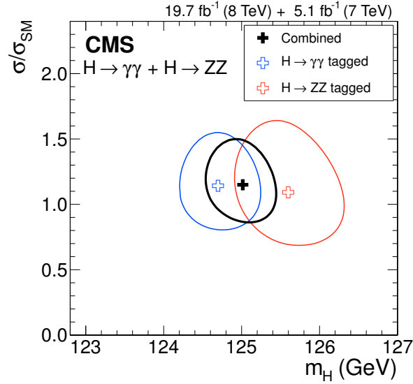
Figure 1: The 68% CL confidence regions for the signal strength \sigma/\sigma_{\text{SM}} versus the mass of the boson m_H for the H \rightarrow \gamma\gamma and H \rightarrow ZZ \rightarrow 4\ell final states, and their combination. The symbol \sigma/\sigma_{\text{SM}} denotes the production cross section times the relevant branching fractions, relative to the SM expectation. In this combination, the relative signal strength for the two decay modes is set to the expectation for the SM Higgs boson.
