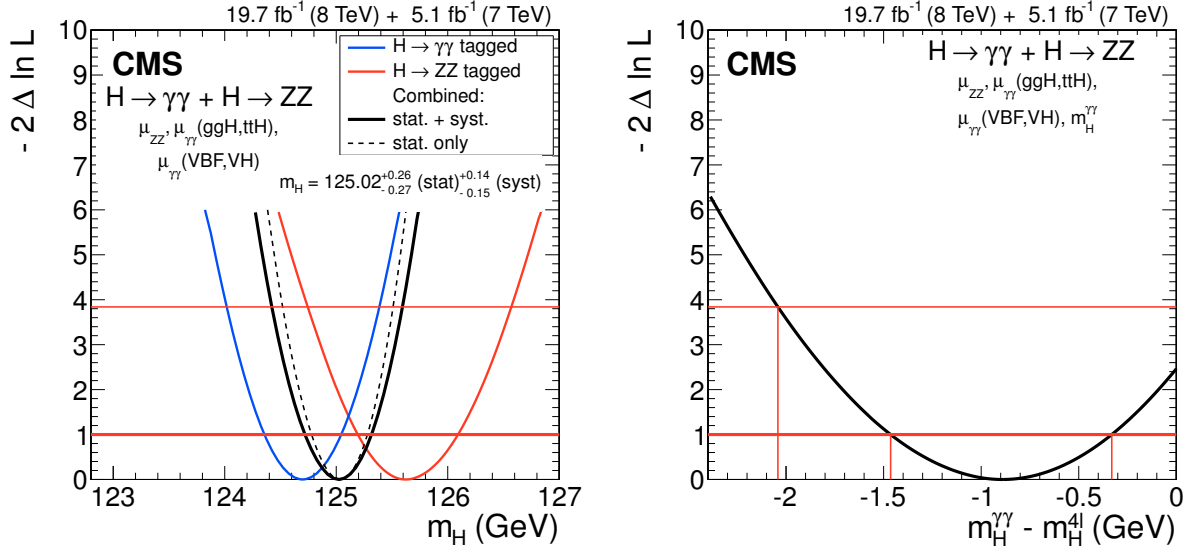
Figure 2: (Left) Scan of the test statistic q(m_H) = -2\Delta\ln\mathcal{L} versus the mass of the boson m_H for the H \rightarrow \gamma\gamma and H \rightarrow ZZ \rightarrow 4\ell final states separately and for their combination. Three independent signal strengths, (ggH, ttH) \rightarrow \gamma\gamma , (VBF, VH) \rightarrow \gamma\gamma , and pp \rightarrow H \rightarrow ZZ \rightarrow 4\ell , are profiled together with all other nuisance parameters. (Right) Scan of the test statistic q(m_H^{\gamma\gamma} - m_H^{4\ell}) versus the difference between two individual mass measurements for the same model of signal strengths used in the left panel.
