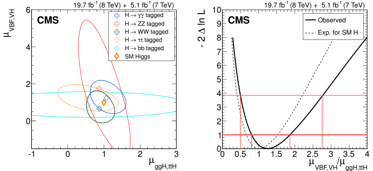
Figure 5: (Left) The 68% CL confidence regions (bounded by the solid curves) for the signal strength of the ggH and ttH and of the VBF and VH production mechanisms, \mu_{\text{ggH},\text{ttH}} and \mu_{\text{VBF},\text{VH}} , respectively. The crosses indicate the best-fit values obtained in each group of predominant decay modes: \gamma\gamma , ZZ, WW, \tau\tau , and bb. The diamond at (1, 1) indicates the expected values for the SM Higgs boson. (Right) Likelihood scan versus the ratio \mu_{\text{VBF},\text{VH}}/\mu_{\text{ggH},\text{ttH}} , combined for all channels. The fit for \mu_{\text{VBF},\text{VH}}/\mu_{\text{ggH},\text{ttH}} is performed while profiling the five \mu_{\text{ggH},\text{ttH}} parameters, one per visible decay mode, as shown in Table 4. The solid curve represents the observed result in data while the dashed curve indicates the expected median result in the presence of the SM Higgs boson. Crossings with the horizontal thick and thin lines denote the 68% CL and 95% CL confidence intervals, respectively.
