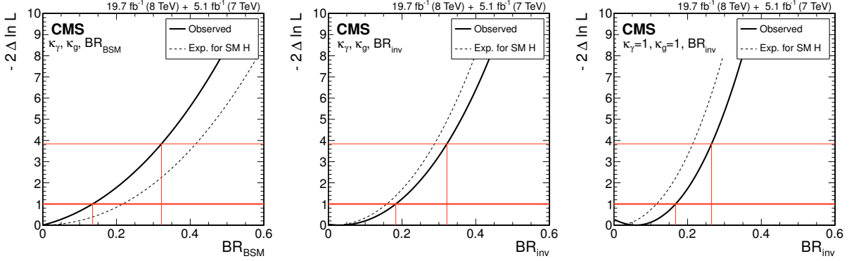
Figure 15: (Left) The likelihood scan versus BR_{BSM} = \Gamma_{BSM}/\Gamma_{tot} . The solid curve represents the observation and the dashed curve indicates the expected median result in the presence of the SM Higgs boson. The partial widths associated with the tree-level production processes and decay modes are assumed to be as expected in the SM. (Middle) Result when also combining with data from the H(inv) searches, thus assuming that BR_{BSM} = BR_{inv} , i.e. that there are no undetected decays, BR_{undet} = 0 . (Right) Result when further assuming that \kappa_g = \kappa_\gamma = 1 and combining with the data from the H(inv) searches.
