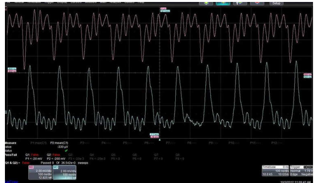
Figure 7: The time structure of MCP1 (upper signal) and photodiode (low signal).
