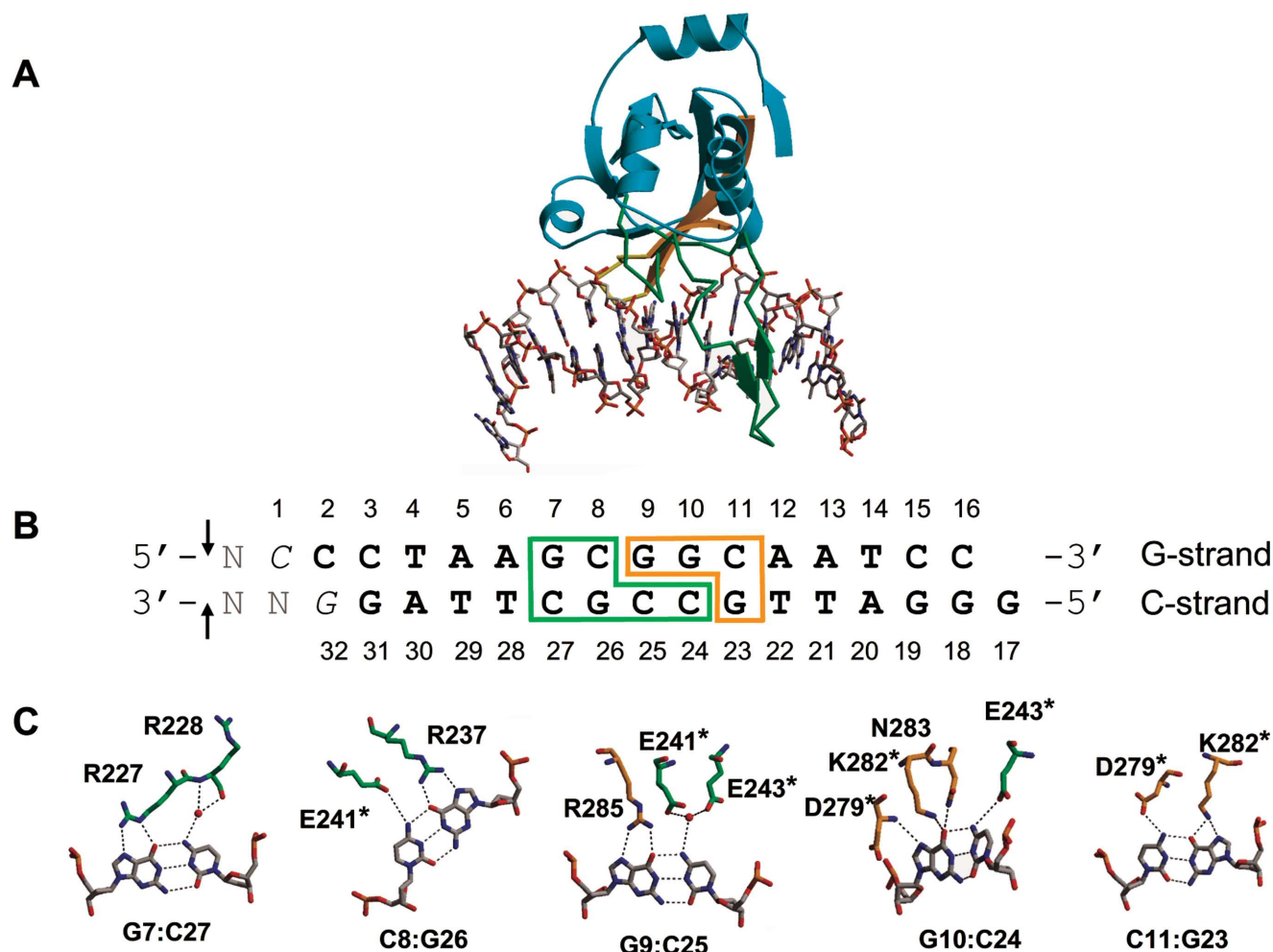
Figure 2. DNA recognition by R.NgoAVII-B3. (A) Overall structure of the complex. The N-arm (residues 247–264) is colored green and the C-arm (residues 290–303) is colored orange. (B) The cognate oligoduplex DNA-1 used in co-crystallization. The DNA bases of the recognition site are boxed green and orange depending on whether they are recognized by the N-arm or C-arm, respectively. Nucleotides C1 and G32 (shown in italic) are not visible in the structure. The 'N' nucleotides (gray) are added to mark the NgoAVII cleavage sites shown by the arrows (8). To simplify the comparison of DNA binding and recognition patterns between R.NgoAVII-B3 and BfiI/EcoRII B3-like domains, we kept the conserved orientation of the N- and C-arms, therefore the recognition sequence 5'-GCCGC-3' of R.NgoAVII is shown in the opposite direction. This flip of the recognition sequence conditionally positions the cleavage site on the opposite side of the target sequence. (C) Recognition of the individual base pairs by R.NgoAVII-B3. Residues from the N-arm are colored green and residues from the C-arm are colored orange. Residues involved in the recognition of more than one base pair are marked by asterisk.
