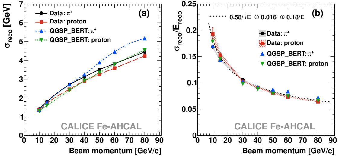
Figure 7. (a) Absolute and (b) fractional energy resolution for pions (black circles), protons (red squares), simulated pions (blue triangles), and simulated protons (green down triangles) using the QGSP_BERT physics list. Error bars show the statistical uncertainties. The grey and crosshatched red bands show the systematic uncertainties for pion and proton data, respectively (not estimated for the absolute resolution).
