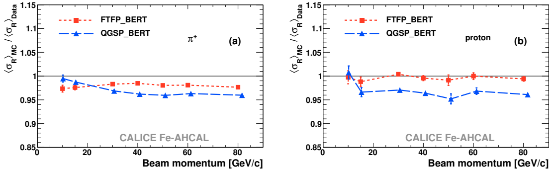
Figure 17. Ratio of the mean radial dispersion from simulations using the FTFP_BERT (red squares) and QGSP_BERT (blue triangles) physics lists to data for (a) pion and (b) proton-induced showers. Data are corrected for bias as described in Section 2.4.
