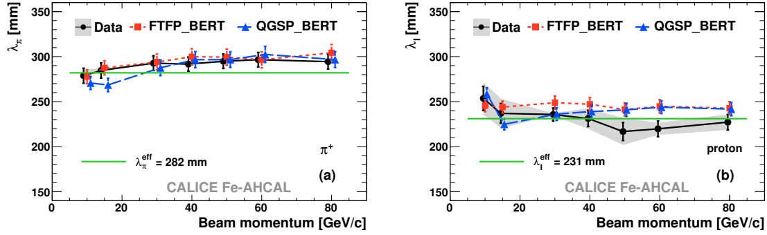
Figure 1. Nuclear interaction length (a) \lambda_{\pi} for pions and (b) \lambda_l for protons in the CALICE Fe-AHCAL extracted from found shower start for data samples (black circles) and simulations using the FTFP_BERT (red squares) and QGSP_BERT (blue triangles) physics lists of GEANT4 9.6. Error bars show the uncertainties from fit. The green solid line corresponds to the effective nuclear interaction length calculated from PDG data. Systematic uncertainties for data are shown with a grey band (not visible in the left plot).
