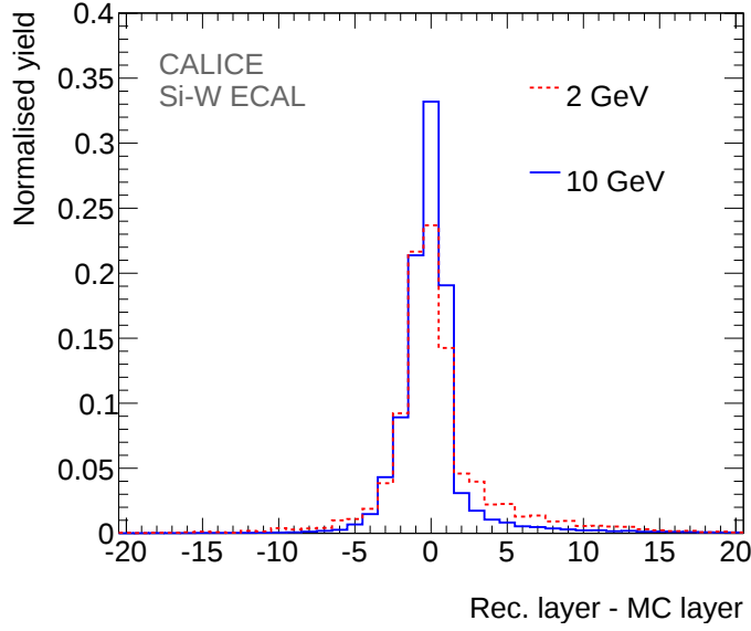
Figure 5: The difference between the reconstructed and the true interaction layers found with the physics list FTFP_BERT for \pi^- of 2 and 10 GeV.
