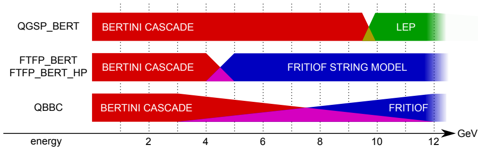
Figure 2: Model used for hadronic interactions of \pi^- depending on the physics list and the energy of the interacting particle.
