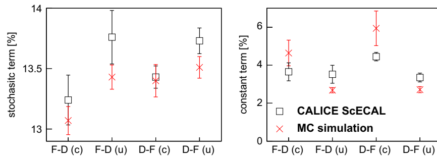
Fig. 16. Comparison of the stochastic (left) and constant (right) terms of the energy resolution measured in data and simulations in the central (“c”) and uniform (“u”) regions of both detector configurations. The beam energy spread has neither been subtracted from the data, nor included in the simulations. The error bars on the data correspond to the quadratic sum of the statistical uncertainty and all systematic uncertainties except that due to the beam energy spread. The error bars on the simulation points include the statistical uncertainty and systematic effects related to the strip attenuation length.
