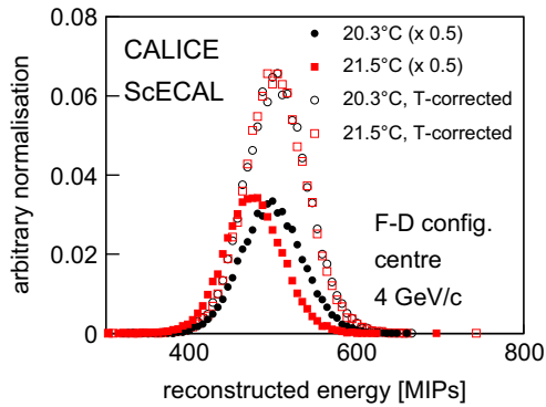
Fig. 10. The measured energy distributions of EM shower data in two runs at a beam momentum of 4 GeV/c. The closed (open) symbols show the response before (after) the application of the temperature correction. The uncorrected curves have been scaled by 50% to aid visibility. (The cross-talk correction has not been applied.)
