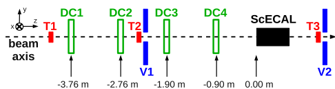
Fig. 6. Sketch of the beam line instrumentation, showing the layout of the four pairs of drift chambers (DC1–4), three trigger counters (T1–3) and the two veto counters (V1–2) relative to the ScECAL prototype. (Not to scale.)
