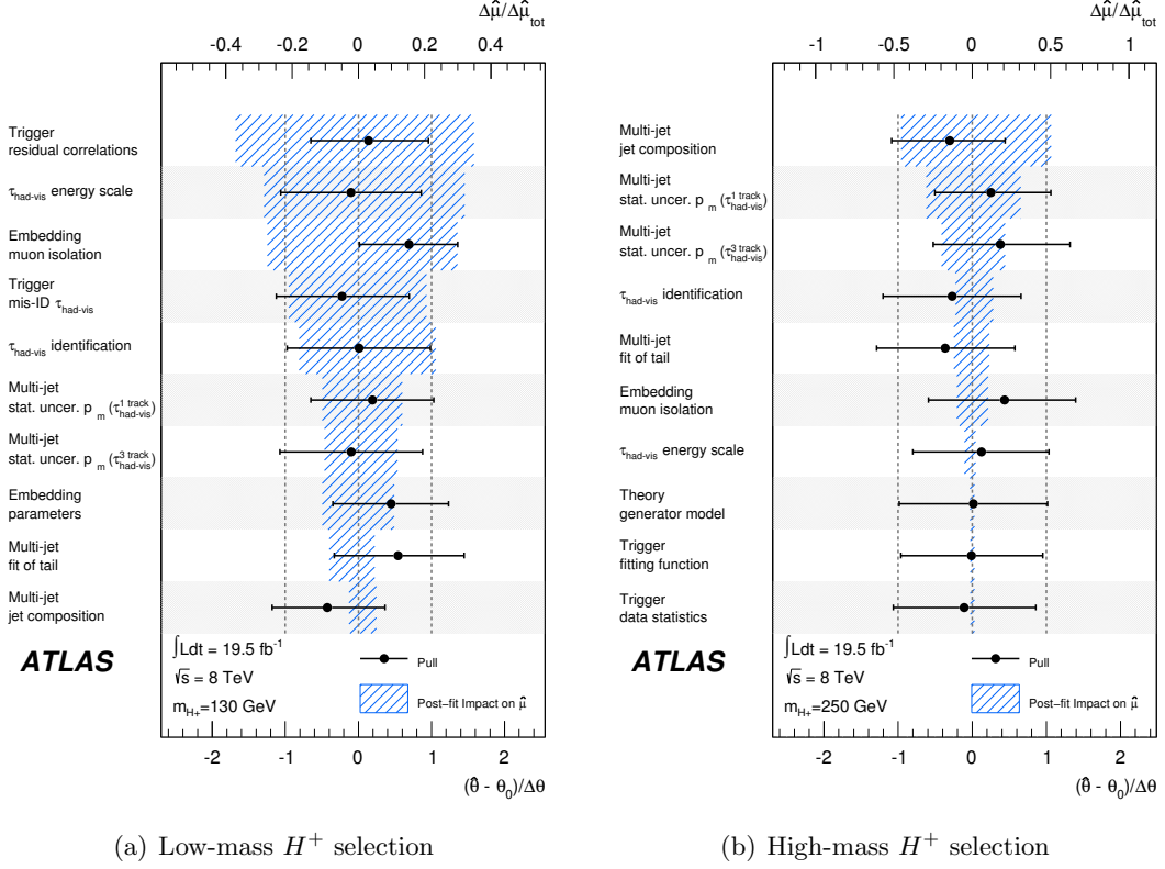
Figure 5. Impact of systematic uncertainties on the final observed limits for (a) m_{H^+} = 130 GeV and (b) m_{H^+} = 250 GeV. The systematic uncertainties are ordered (top to bottom) by decreasing impact on the fitted signal strength parameter. The dots, which refer to the bottom horizontal axis, show how each fitted nuisance parameter, \hat{\theta} , deviates from its nominal value, \theta_0 , in terms of standard deviations with respect to its nominal uncertainty, \Delta\theta . The solid lines indicate the post-fit uncertainties of each nuisance parameter, also relative to their nominal values. The hatched band, referring to the top horizontal axis, shows the deviations of the fitted signal-strength parameter after changing a specific nuisance parameter upwards or downwards by its post-fit uncertainty ( \Delta\hat{\mu} ) as a fraction of the total uncertainty of the fitted signal-strength parameter ( \Delta\hat{\mu}_{\text{tot}} ).
