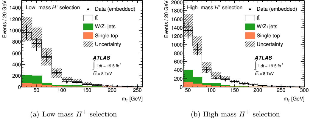
Figure 2. Comparison of the m_T distributions for events with a true \tau_{\text{had}} for the (a) low-mass and (b) high-mass charged Higgs boson search, as predicted by the embedding method and simulation. Combined statistical and systematic uncertainties (as described in section 5) for the embedded sample are shown as error bars, and all systematic uncertainties applicable to simulation are shown as hatched bands.
