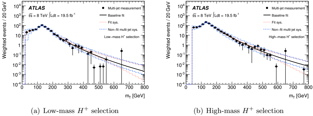
Figure 3. The multi-jet background predictions from data-driven methods for the (a) low-mass and (b) high-mass H^+ event selections, with the results of fits using the power-log function, are shown in the solid line. The dotted lines show the systematic uncertainty from the choice of the fit function. The dashed lines show the total combined fits from the sources of systematic uncertainty listed in table 4.
