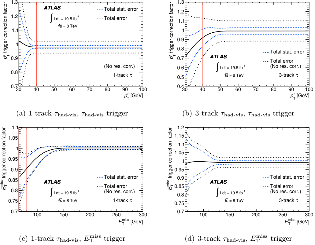
Figure 4. Inclusive \tau_{\text{had-vis}} and E_T^{\text{miss}} trigger correction factors obtained from the ratio of functions fitted to data and simulation for \tau_{\text{had-vis}} with (a,c) one and (b,d) three charged tracks are shown at the top and bottom, respectively. The vertical line on the \tau_{\text{had-vis}} trigger correction factor plots indicates the lowest p_T^\tau threshold used in the analysis. The vertical line on the E_T^{\text{miss}} trigger correction factor plots shows the lower boundary used in the high-mass charged Higgs boson search. The total statistical uncertainty is indicated with the dotted line and the systematic uncertainty is added in quadrature to the statistical error (dashed-dotted line). For \tau_{\text{had-vis}} trigger efficiencies, the total systematic uncertainty is shown, while for the E_T^{\text{miss}} trigger efficiency, the systematic uncertainty related to residual correlations between \tau_{\text{had-vis}} and E_T^{\text{miss}} is not included, since the effect is evaluated separately for several signal mass ranges and background samples.
