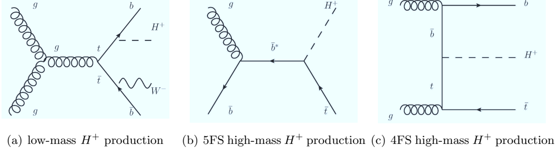
Figure 1. Leading-order Feynman diagrams for the dominant production modes of charged Higgs bosons at masses (a) below and (b, c) above the top-quark mass.
