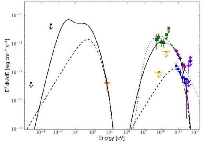
Fig. 7. Spectral energy distribution (SED) for three different assumptions about the nature of the source. Solid line: The association between a single TeV source (violet diamonds) and the GeV source (green squares) has been assumed. A leptonic scenario has been tested where a low-energy Maxwellian distribution replaces the low-energy part of the electron spectrum. The fitted parameters of this model can be found in Table 3. Dashed line: a simple leptonic model has been tested assuming the TeV point-like source (blue points) is associated with a hypothetical GeV point-like source superimposed on the extended one (yellow upper limits). The blue TeV spectral points have been obtained after normalizing the points computed in the central extracted region (see Sect. 2.2 for details). Dash-dotted line: the hadronic model studied by Li & Chen (2012) has been superimposed to the new data points obtained in this work. The brown X-ray spectral point has been derived from the XMM-Newton spectrum given by Mukherjee et al. (2009), the black radio upper limits from VLA 20 cm (Helfand et al. 2006) and Bolocam 1.1 mm (Aguirre et al. 2011) images.
