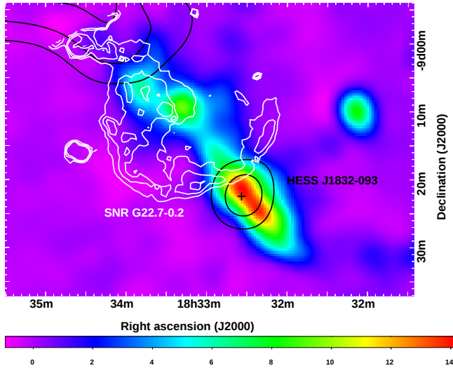
Figure 4. Integrated ^{13}\text{CO} antenna temperature in arbitrary units (Jackson et al. 2006) in a velocity range of 26 to 31 \text{ km s}^{-1} smoothed with the average H.E.S.S. PSF for this data set. The gamma-ray excess of Fig. 1 is shown in black contours (50, 75 and 100 gamma levels) while the radio observation of SNR G22.7–0.2 (Helfand et al. 2006) at 1.4 GHz is overlaid in white contours. (0.002 and 0.005 mJy/beam). The black cross represents the best-fit position of the H.E.S.S. excess with corresponding errors.
