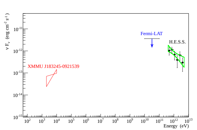
Figure 2. Spectral energy distribution from the region of VHE emission from HESS J1832–093. The VHE gamma-ray spectrum observed with H.E.S.S. is displayed together with the upper limit obtained between 10 and 100 GeV with the Fermi-LAT. The green contour represents the 1\sigma confidence level of the fitted spectrum using a power-law hypothesis. Only statistical errors (68% confidence level) are shown for the spectral points. The X-ray power-law model of XMMU J183245–0921539 is overlaid in red, taking into account the statistical uncertainties only.
