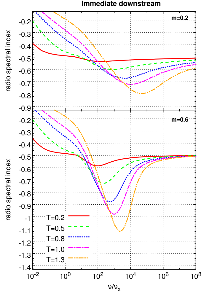
Fig. 6. Radio spectral index of the shell where reacceleration occurs, plotted for different times T and 2 choices of m .
