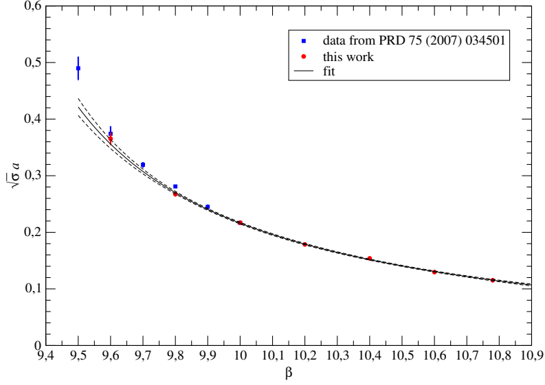
Figure 2. Results for the square root of the string tension in lattice units, as a function of the Wilson action parameter \beta . The plot shows our simulation results (red circles) in comparison with those from ref. [81] (blue squares), as well as the interpolating function described by eq. (3.1) for the values of the parameters listed in the text (solid black curve), with the associated uncertainty (dashed black curves).
