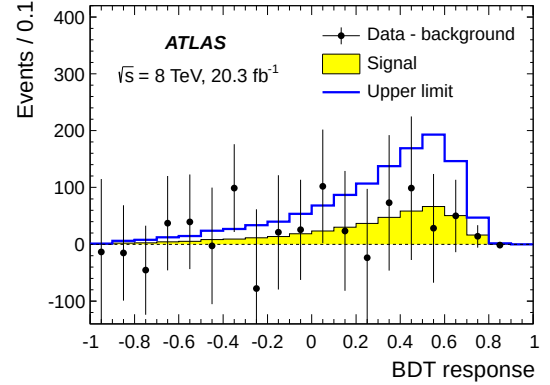
Figure 3: Observed and predicted (filled histogram) signal distributions of the BDT response after background subtraction. The signal and subtracted simulated background contributions are normalized to the result of the binned maximum-likelihood fit. The error bars represent the statistical uncertainty of the data added in quadrature with the simulation statistical uncertainties and with the systematic uncertainties on the background normalizations described in Section 7. The empty histogram represents the predicted signal distribution renormalized to the observed cross-section upper limit reported in Section 9.
