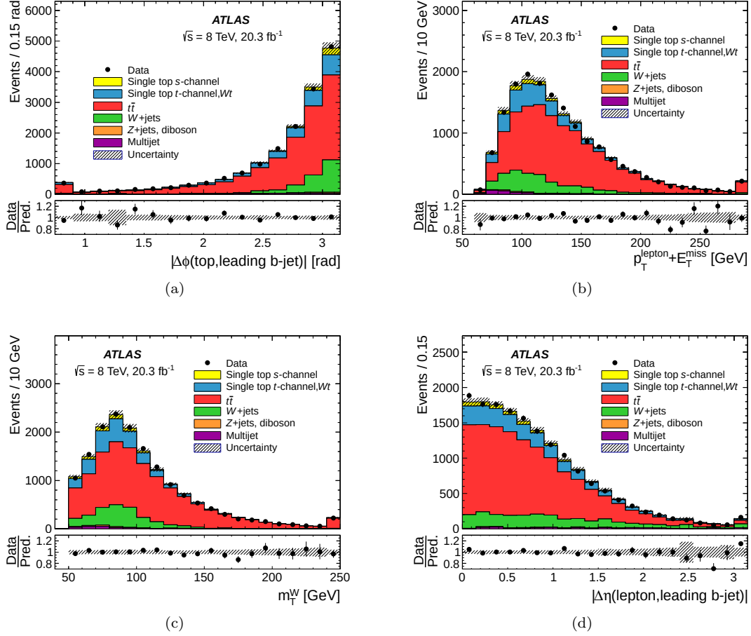
Figure 1: Observed and predicted distributions in the signal region of four of the most discriminating variables used in the BDT classifier (a) azimuthal angle between the leading b -jet and the top-quark reconstructed with the sub-leading b -jet, (b) scalar sum of the lepton momentum and the missing transverse momentum, (c) W boson transverse mass, and (d) difference in pseudorapidity between the lepton and the leading b -jet. The simulated distributions are normalized to the result of the binned maximum-likelihood fit described in Section 8. The hatched bands represent the normalization uncertainty of all processes after the fit added in quadrature with the simulation statistical uncertainty. The lower panels show the ratio of data to prediction. The first (last) bin of the histograms includes underflows (overflows).
