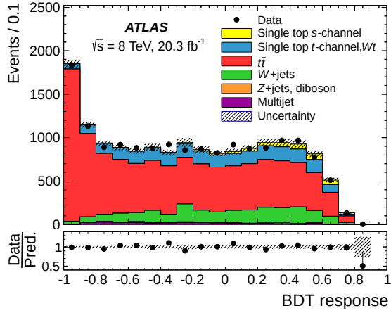
Figure 2: Observed and predicted distributions of the BDT response. The simulated distributions are normalized to the result of the binned maximum-likelihood fit. The hatched band represents the normalization uncertainty of all processes after the fit added in quadrature with the simulation statistical uncertainty. The lower panel shows the ratio of data to prediction.
