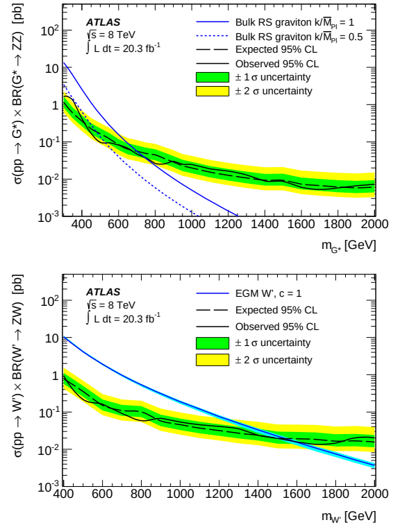
Fig. 2 Observed and expected 95% CL upper limits on the cross section times branching fraction as a function of the resonance pole mass for the G^* (top) and EGM W' (bottom). The LO (NNLO) theoretical cross sections for G^* ( EGM W' ) production with k/\bar{M}_{Pl} = 0.5 and 1.0 ( c = 1 ) are also shown. The band around the W' cross section represents the theoretical uncertainty on the NNLO calculation. The inner and outer bands on the expected limits represent \pm 1\sigma and \pm 2\sigma variations respectively.
