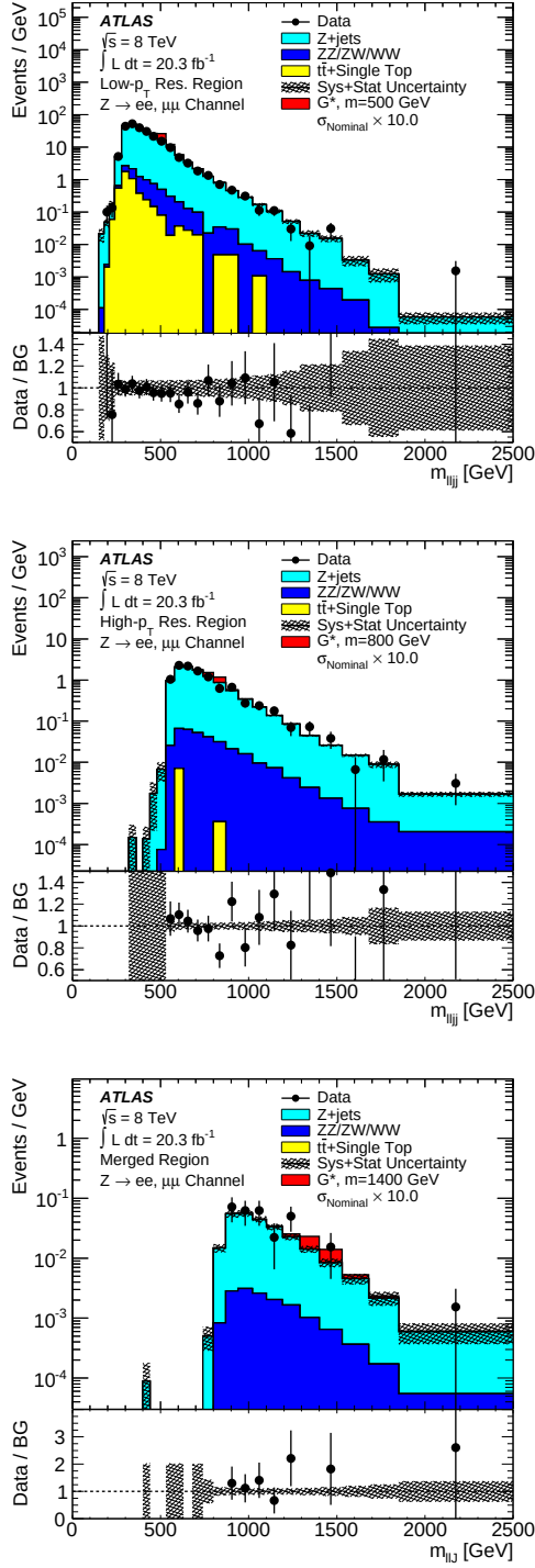
Fig. 1 Reconstructed \ell\ell jj or \ell\ell J mass distributions in the data and for background after all the selection cuts are applied in the three kinematic regions referred to as the LR (top), HR (middle) and MR (bottom) in the text. The shaded regions show the full background uncertainty obtained by adding statistical and systematic uncertainties in quadrature, including the constraints on the background from the data control regions and before the fit to the data in the signal regions (cf. unconstrained case in Table 2). Also shown are the G^* signal yields expected for masses of 500, 800 and 1400 GeV with the production cross sections scaled by a factor 10.
