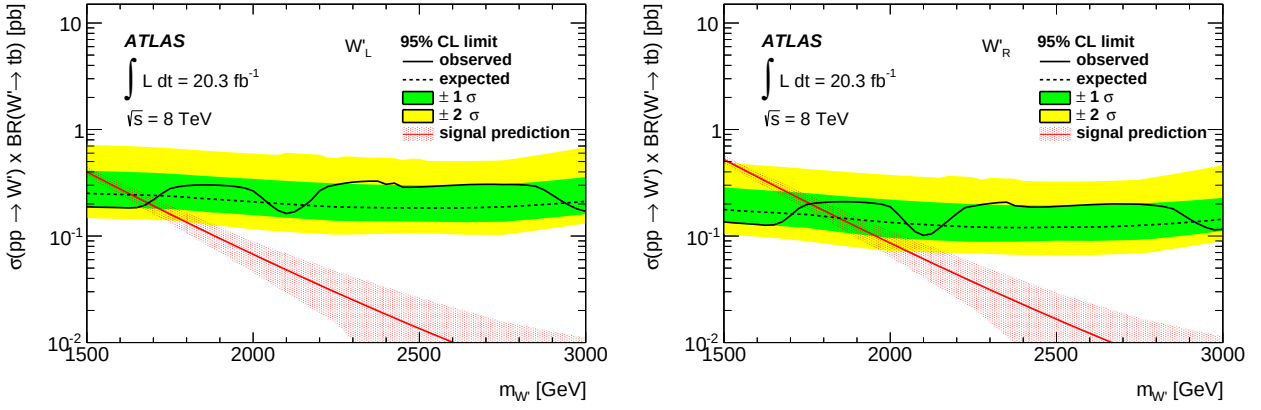
Fig. 6: Limits at 95% CL on the cross section times branching ratio to tb for the left-handed (left) and for the right-handed (right) W' model. The expected cross section for W' production with g' = g_{\text{SM}} is also shown.
