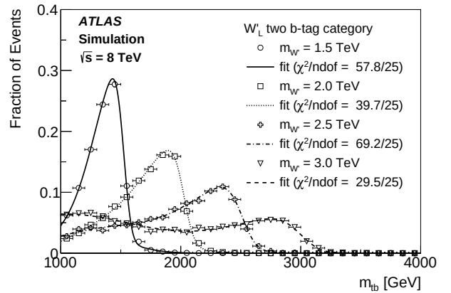
Fig. 2: Parametric fits to the W' \rightarrow tb \rightarrow qqbb signal distributions in the two b -tag category for W'_L masses between 1.5 and 3 TeV overlaid to the corresponding MC distributions. While unbinned fits are performed, the events from MC simulation are shown as a histogram for presentational purposes.
