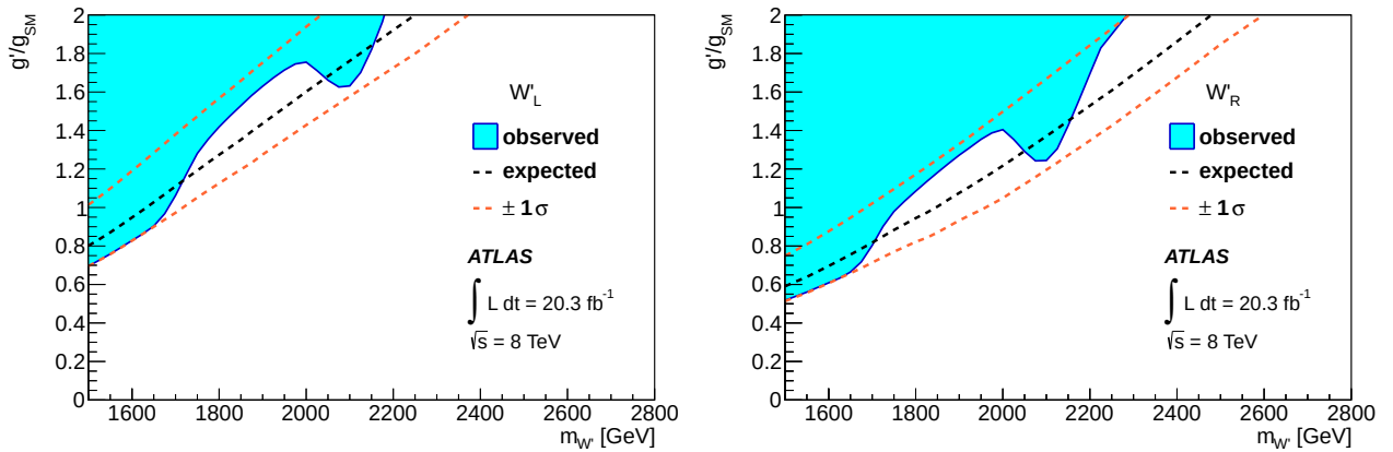
Fig. 7: Observed and expected 95% CL limits on the ratio of coupling g'_L/g_{\text{SM}} ( g'_R/g_{\text{SM}} ) of the W'_L ( W'_R ) model as a function of the W' mass.
