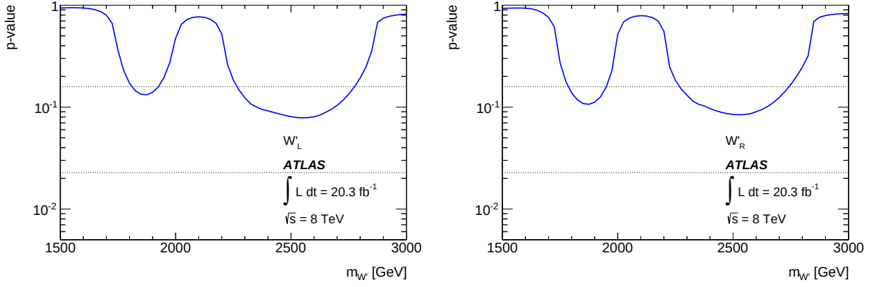
Fig. 5: Observed p -values for a left-handed (left) and right-handed (right) W' model as a function of the W' mass.
