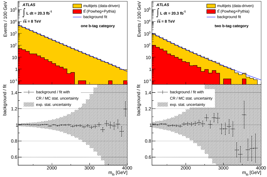
Fig. 3: Fit to the m_{tb} distribution from the initial background estimate in the one b -tag category (left) and in the two b -tag category (right). The ratio background/fit is also shown, where the uncertainties are the control-region and MC statistical uncertainties and the grey shaded band shows the statistical uncertainty in each bin as expected for 20.3 \text{ fb}^{-1} .
