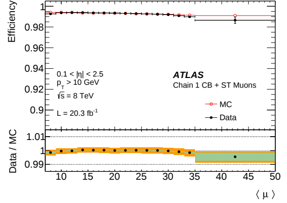
Fig. 6. Measured CB+ST muon reconstruction efficiency for muons with p_T > 10 GeV as a function of the average number of inelastic pp collisions per bunch crossing (the \langle \mu \rangle parameter). The error bars on the efficiencies indicate the statistical uncertainty. The panel at the bottom shows the ratio between the measured and predicted efficiencies. The green areas depict the pure statistical uncertainty, while the orange areas also include systematic uncertainties.
