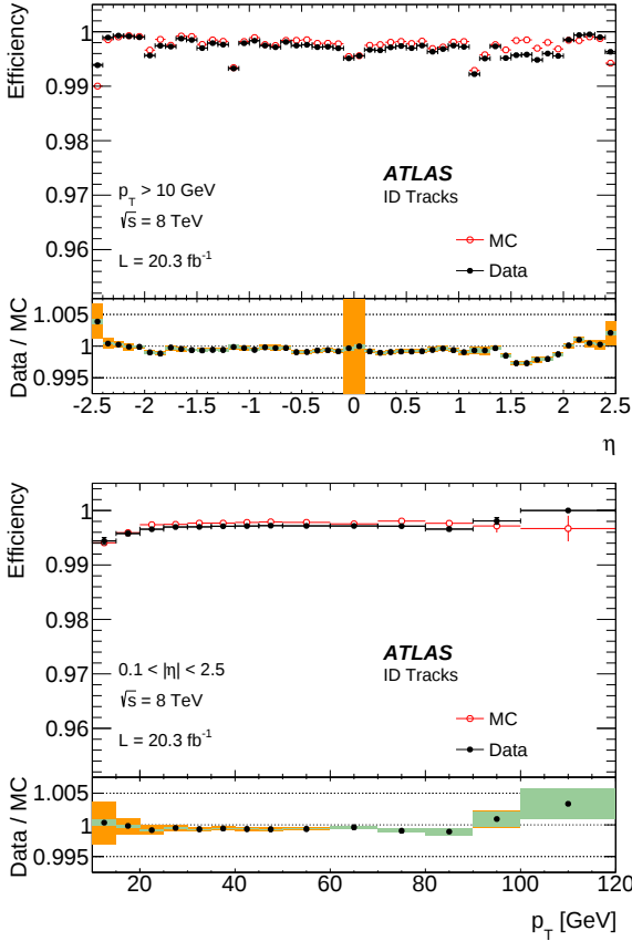
Fig. 4. ID muon reconstruction efficiency as a function of \eta (top) and p_T (bottom) measured in Z \rightarrow \mu\mu events for muons with p_T > 10 GeV. The error bars on the efficiencies indicate the statistical uncertainty. The panel at the bottom shows the ratio between the measured and predicted efficiencies. The green areas depict the pure statistical uncertainty, while the orange areas also include systematic uncertainties.
