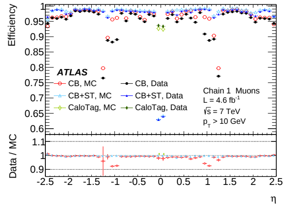
Fig. 19. Muon reconstruction efficiency as a function of \eta measured in Z \rightarrow \mu\mu events in the 2011 data sample for different muon reconstruction types. CaloTag muons are only shown in the region |\eta| < 0.1 , where they are used in physics analyses. For the efficiency, the error bars indicate the statistical uncertainty. The panel at the bottom shows the ratio between the measured and MC efficiencies. The error bars on the ratios show the combination of statistical and systematic uncertainties. The lower efficiency of CB muons at |\eta| \approx 1.2 is due to the fact that some of the MS chambers were not yet installed.
