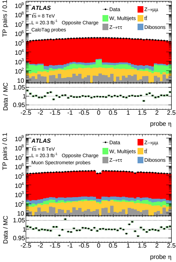
Fig. 1. Pseudorapidity distribution of the CaloTag (top) or MS (bottom) probes used in the “tag and probe” analysis. The bottom panel shows the ratio between observed and expected counts. The sum of the MC samples is normalized to the number of events in the data. The green band represents the statistical uncertainty.
