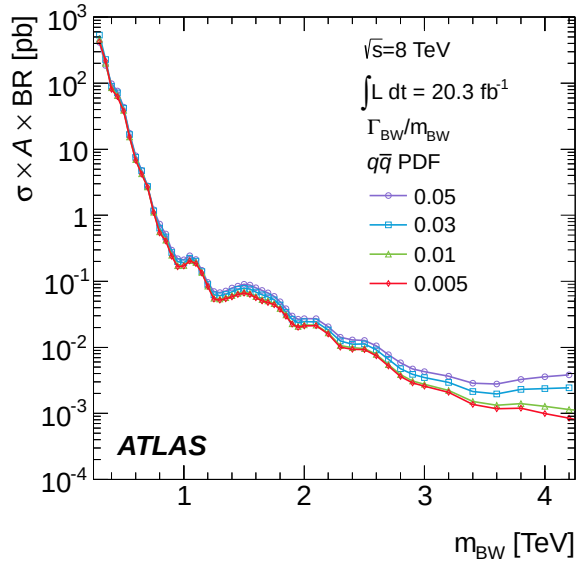
Figure 10. The 95% CL upper limits on \sigma \times \mathcal{A} for a Breit–Wigner narrow resonance produced by a q\bar{q} initial state decaying to dijets and convolved with PDF effects, dijet mass acceptance and detector resolution as a function of the mean mass, m_{BW} , for different values of intrinsic width over mass ( \Gamma_{BW}/m_{BW} ), taking into account both the statistical and systematic uncertainties.
