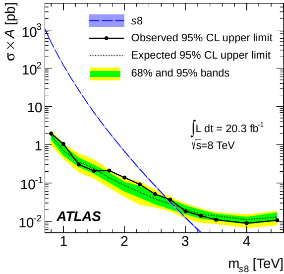
Figure 4. Observed (filled circles) and expected 95% CL upper limits (dotted line) on \sigma \times \mathcal{A} for color-octet scalars as a function of particle mass. The green and yellow bands represent the 68% and 95% contours of the expected limit. The dashed curve is the theoretical prediction of \sigma \times \mathcal{A} . The uncertainty on the nominal signal cross section due to the beam energy uncertainty is also displayed as a band around the theory prediction. The observed (expected) mass limit occurs at the crossing of the dashed \sigma \times \mathcal{A} curve with the observed (expected) 95% CL upper limit curve.
