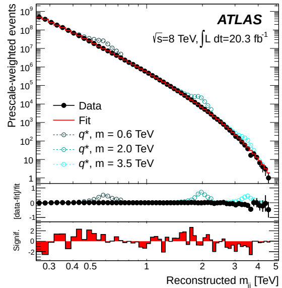
Figure 2. The reconstructed dijet mass distribution (filled points) fitted with a smooth functional form (solid line). Predictions for three q^* masses are shown above the background. The central panel shows the relative difference between the data and the background fit with overlaid predictions for the same q^* masses. The bin-by-bin significance of the data-background difference is shown in the bottom panel.
