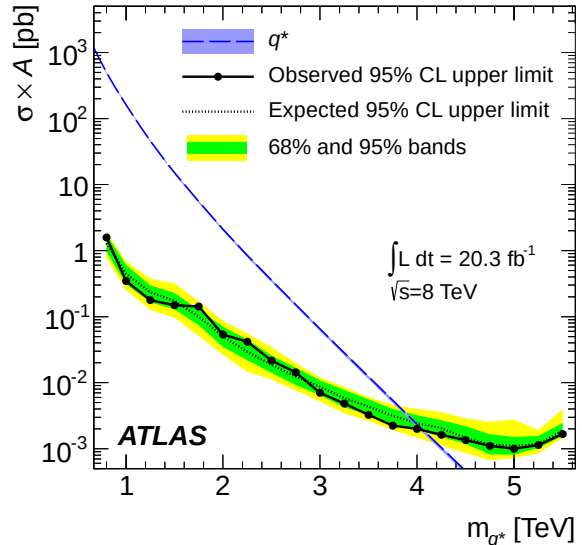
Figure 3. Observed (filled circles) and expected 95% CL upper limits (dotted line) on \sigma \times \mathcal{A} for excited quarks as a function of particle mass. The green and yellow bands represent the 68% and 95% contours of the expected limit. The dashed curve is the theoretical prediction of \sigma \times \mathcal{A} . The uncertainty on the nominal signal cross section due to the beam energy uncertainty is also displayed as a band around the theory prediction. The observed (expected) mass limit occurs at the crossing of the dashed \sigma \times \mathcal{A} curve with the observed (expected) 95% CL upper limit curve.
