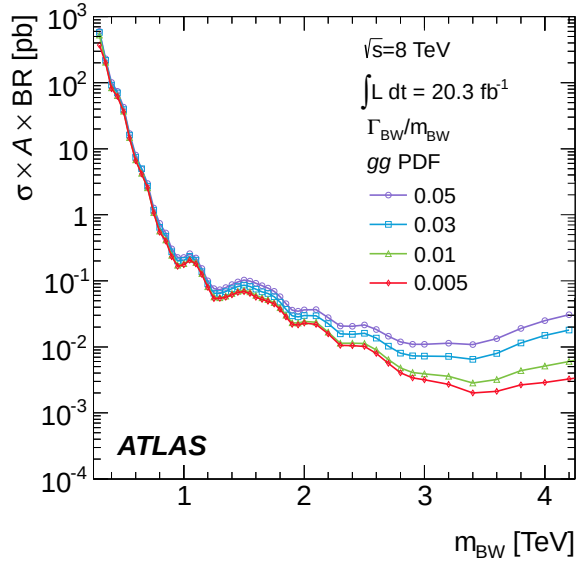
Figure 9. The 95% CL upper limits on \sigma \times \mathcal{A} for a Breit–Wigner narrow resonance produced by a gg initial state decaying to dijets and convolved with PDF effects, dijet mass acceptance and detector resolution as a function of the mean mass, m_{BW} , for different values of intrinsic width over mass ( \Gamma_{BW}/m_{BW} ), taking into account both the statistical and systematic uncertainties.
