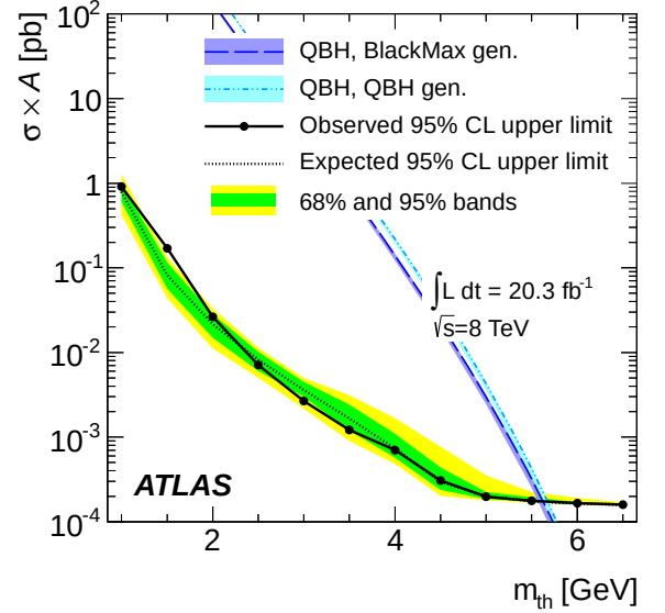
Figure 7. Observed (filled circles) and expected 95% CL upper limits (dotted line) on \sigma \times \mathcal{A} for black holes simulated using the QBH and BLACKMAX generators as a function of particle mass. The green and yellow bands represent the 68% and 95% contours of the expected limit. The dashed curve is the theoretical prediction of \sigma \times \mathcal{A} . The uncertainty on the nominal signal cross section due to the beam energy uncertainty is also displayed as a band around the theory prediction. The observed (expected) mass limit occurs at the crossing of the dashed \sigma \times \mathcal{A} curve with the observed (expected) 95% CL upper limit curve.
