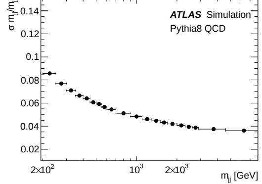
Figure 11. Dijet mass resolution obtained from fully simulated PYTHIA QCD Monte Carlo PYTHIA 8.175 [43], with the AU2 tune obtained from ATLAS data [45]. The dijet mass resolution is interpolated linearly between the bin centers.
