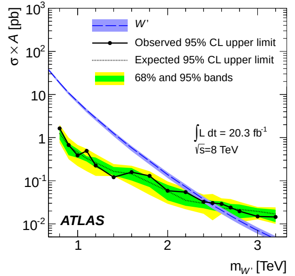
Figure 5. Observed (filled circles) and expected 95% CL upper limits (dotted line) on \sigma \times \mathcal{A} for heavy vector bosons as a function of particle mass. The green and yellow bands represent the 68% and 95% contours of the expected limit. The dashed curve is the theoretical prediction of \sigma \times \mathcal{A} . The uncertainty on the nominal signal cross section due to the beam energy uncertainty is also displayed as a band around the theory prediction. Additionally the uncertainty on the calculation of the next-to-next-to-leading order cross section is shown around the theory line. The observed (expected) mass limit occurs at the crossing of the dashed \sigma \times \mathcal{A} curve with the observed (expected) 95% CL upper limit curve.
