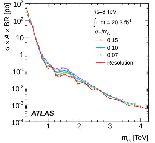
Figure 8. The 95% CL upper limits on \sigma \times \mathcal{A} for a simple Gaussian resonance decaying to dijets as a function of the mean mass, m_G , for four values of \sigma_G/m_G , taking into account both the statistical and systematic uncertainties.
