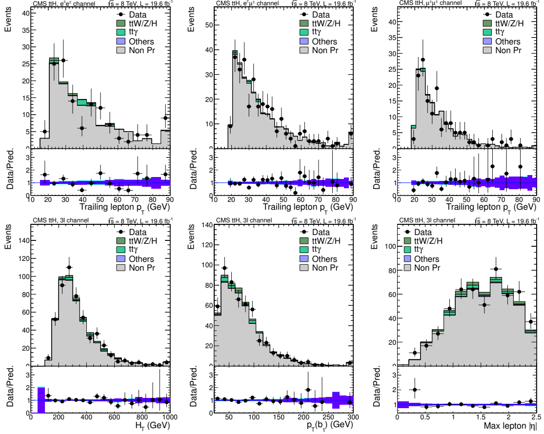
Figure 10. These plots show the distribution of key discriminating variables for events where one lepton fails the lepton MVA requirement. The expected distribution for the non-prompt background is taken from simulation (mostly t\bar{t} +jets), and the yield is fitted from the data. The bottom panel of each plot shows the ratio between data and predictions as well as the overall uncertainties after the fit (blue). In the first row the distributions of the trailing lepton p_T for the e^\pm e^\pm (left), e^\pm \mu^\pm (center), and \mu^\pm \mu^\pm (right) final states are shown. In the second row the distributions of the H_T (left), the p_T of the jet with highest b-tagging discriminator (center), and the lepton maximum |\eta| (right) are shown for the tripleton channel.
