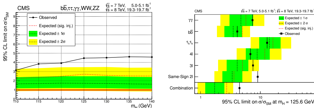
Figure 15. The 95% CL upper limits on the signal strength parameter \mu = \sigma/\sigma_{\text{SM}} . The black solid and dotted lines show the observed and background-only expected limits, respectively. The red dotted line shows the median expected limit for the SM Higgs boson with m_H = 125.6 GeV. The green and yellow areas show the 1\sigma and 2\sigma bands, respectively. Left: limits as a function of m_H for all channels combined. Right: limits for each channel at m_H = 125.6 GeV.
