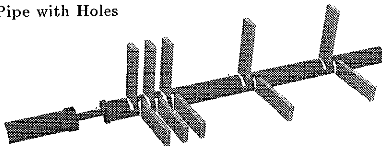
Figure 7. Close-up view of the holes in the beam tube, showing the mesh and the thickness of the beam pipe.
