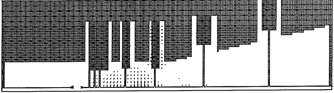
Figure 9. E-Field of the 739.8 MHz mode in the y=0 plane.
