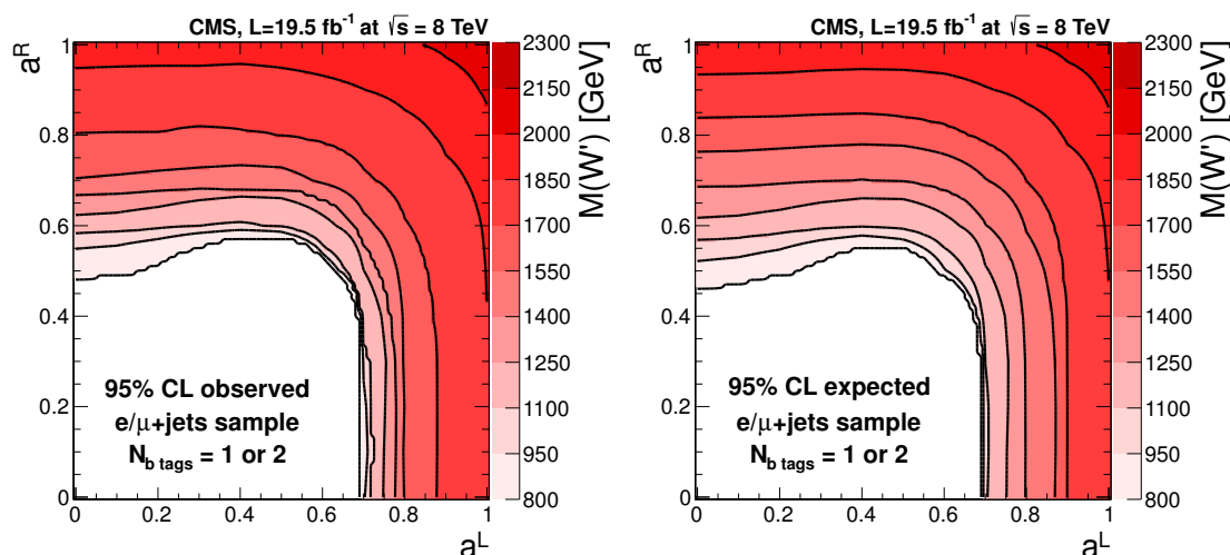
Figure 3. Contour plots of M(W') in the (a^L, a^R) plane for which the 95% CL cross section limit equals the predicted cross section for the combined e, \mu + \text{jets} sample. The left (right) panel represents the observed (expected) limits. The colour axis represents the value of M(W') in GeV. The solid black lines are isocontours of W' -boson mass, plotted in 150 GeV intervals and starting from 800 GeV.
