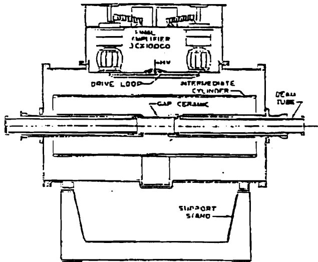
Figure 1. Schematic view of the 52 MHz cavity. Only the beam tube is evacuated. Therefore a ceramic cylinder is placed in the acceleration gap between the ends of the stainless steel drift tubes. This Fig. is taken from [1].
