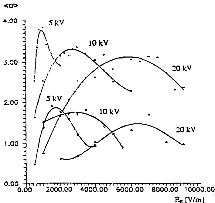
Figure 5. Integral re-emission coefficient \langle \sigma \rangle as a function of the electrostatic field E_c (see text) for three different accelerating voltages. The upper curves stem from the test simulation, the lower ones from the simulation with the "real" fields.
