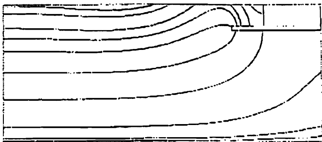
Figure 3. The RF field distribution in the cavity. The field in the region between the ceramic cylinder (upper horizontal line) and the drift tube has been emphasized. The beam axis coincides with the lower horizontal line.
