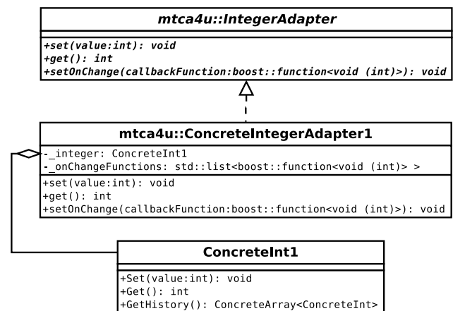
Figure 3: The process variable adapter for an integer type variable. An instance of the concrete control system data type is living within the adapter. Like this there is only a single copy of the data content, which avoids synchronization issues. The control system specific function GetHistory() is intentionally not reflected in the adapter interface.
