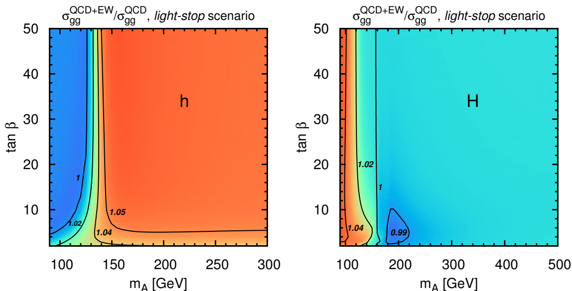
Figure 7. Ratio of gluon-fusion cross section for the production of h (left) and H (right) over the corresponding cross section neglecting EW contributions, as a function of m_A and \tan \beta in the light-stop scenario.
