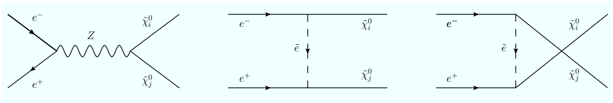
Figure 2: Feynman diagrams for \tilde{\chi}_i^0 \tilde{\chi}_j^0 production at e^+e^- colliders.
