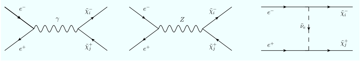
Figure 1: Feynman diagrams for \tilde{\chi}_i^+ \tilde{\chi}_j^- production at e^+e^- colliders.
