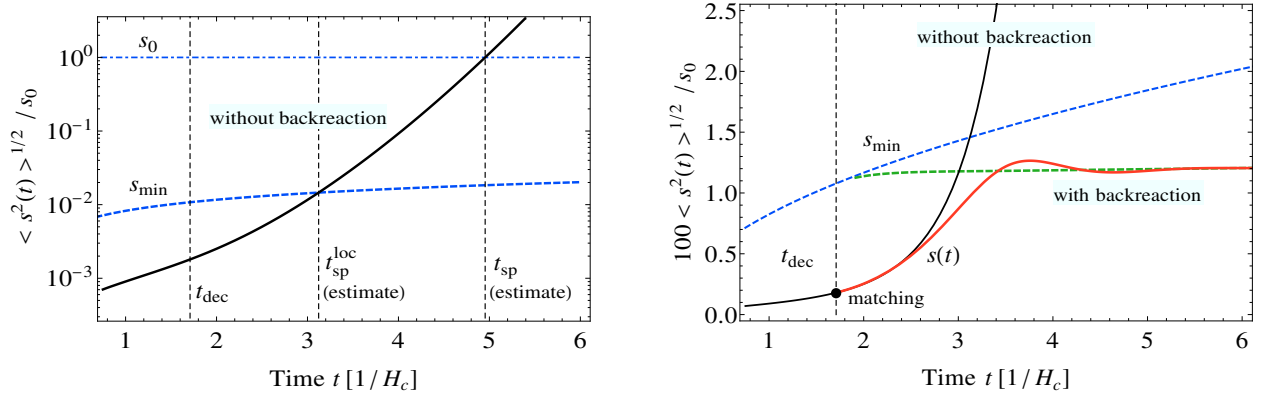
Figure 1: Left (a): Growth of the waterfall field during tachyonic preheating due to quantum fluctuations, comparison with inflaton-dependent minimum s_{\min} in the linear approximation (7) (dashed thick blue) and global minimum s_0 (dashed thin blue) ignoring backreaction effects. Here, we determined the variance \langle s^2(t) \rangle^{1/2} numerically, i.e. by explicitly solving the mode equation for the waterfall field in the relevant k range. Right (b): Classical evolution of the homogeneous waterfall field s(t) after the decoherence time (solid red), comparison with inflaton-dependent minimum including backreaction effects via classical field equations (dashed green). Note that the initial conditions for the evolution of s(t) in the right panel correspond to the numerical values of \langle s^2(t) \rangle^{1/2} and its derivative at t = t_{\text{dec}} in the left panel. Here and in the following figures, the parameter values are: g^2 = 1/2 , \lambda = 5 \times 10^{-4} and \sqrt{\xi} = 2.8 \times 10^{16} GeV.
