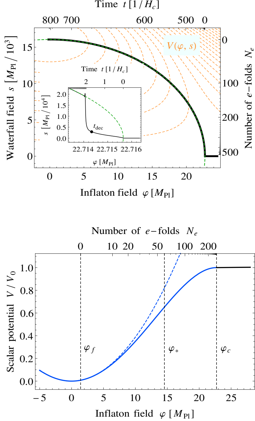
Figure 3: Effective scalar potential during the second stage of inflation. Upper (a): Classical trajectory in two-dimensional field space. Dashed green: analytical solution (17), black: numerical solution from Eqs. (20) and (21). Lower (b): Effective scalar potential for the inflaton field after integrating out the waterfall field. Solid black: Tree-level plus 1-loop potential, solid blue: substituting the waterfall field by its local minimum (17), dashed blue: quadratic approximation.
