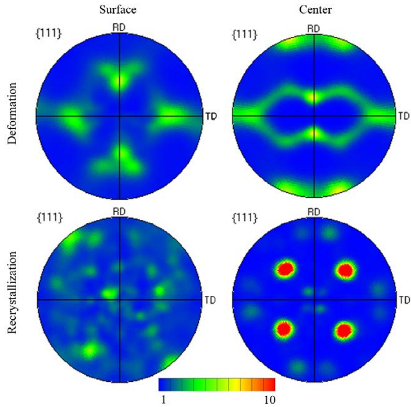
Fig. 4.3: \{111\} pole figures showing the deformation textures of the CI1_95cr sample in the surfaces and the central layer and the recrystallization textures in the surfaces and the central layer.
