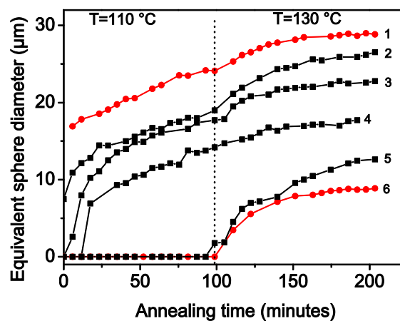
Fig. 5.15: A selection of the measured growth curves of recrystallizing grains in the DPD+CR sample. The red curves represent cube grains, while the black curves represent noncube grains.
