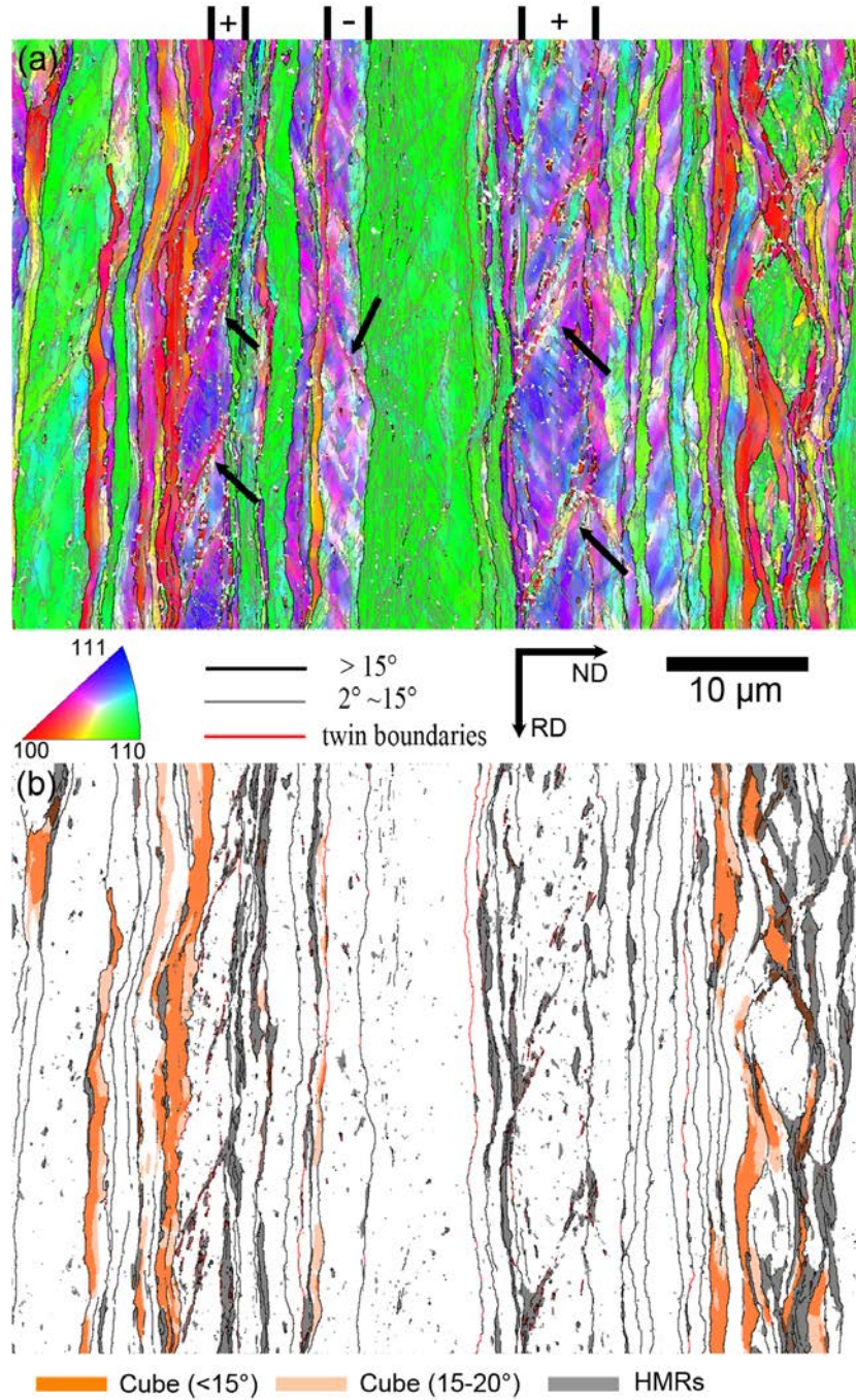
Fig. 4.4: a) Deformation structure of BII, colored according to the crystallographic direction of the ND; both microstructures are composed of bands with different orientations; some bands with localized shear bands (LSBs) are marked, the +/- represents the directions of the LSBs. Further introduction of the +/- pattern can be found in the next paragraph in the main text. Some of the LSBs are indicated by the black arrows. b) The same map as a) with HMRs highlighted in gray, and cube oriented regions in orange; regions of a near cube texture ( 15^\circ - 20^\circ deviation to the ideal cube orientation) are shown in light orange. The LABs are not shown in b).
