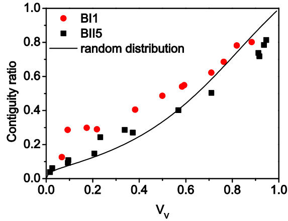
Fig. 4.8: Contiguity ratio C_{aa} as a function of the recrystallized volume fraction V_v for BI1 and BII5. The ITB method was used for this analysis, i.e. annealing twin boundaries are not included as S_{V,aa} . The bold curve shows the theoretical contiguity ratio for randomly distributed recrystallizing grains (Rios et al. 2006).
