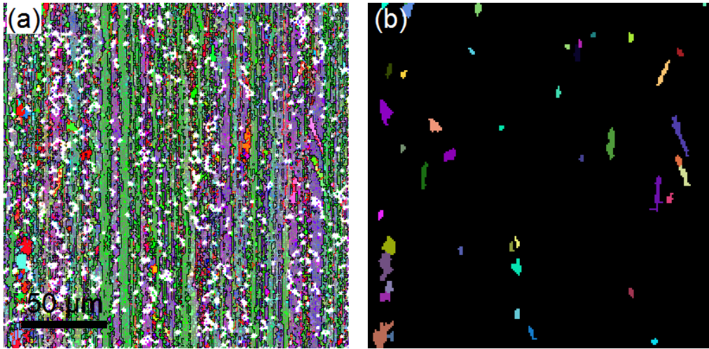
Fig. 4.31: a) Microstructure of BI1_95cr after 30 minutes annealing at 150 °C. The color coding and the sample coordinates are the same those as in Fig. 4.4a. The same map is shown in b) highlighting the recrystallizing grains with random colors. The ITB method was used for grain identification.
