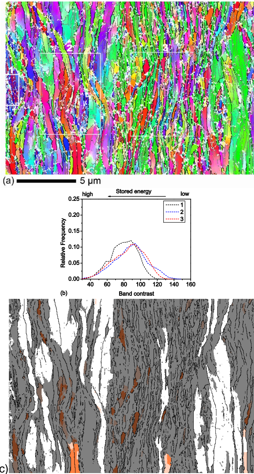
Fig. 5.11: a) Orientation map of the deformation structure of the DPD+CR sample. b) Distributions of band contrasts in framed regions 1/2/3. c) The same map as a) with HMRs, cube and near cube textured regions highlighted. The color coding and the sample coordinates are the same as those in Fig. 4.4.
