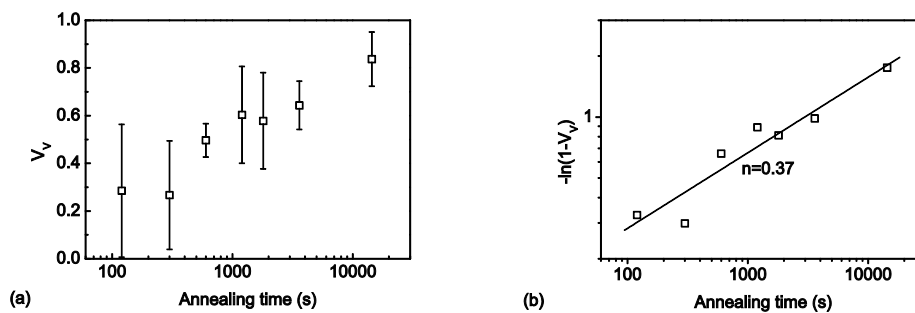
Fig. 5.5: a) Evolution of the recrystallized volume fraction V_V as a function of annealing time for the DPD samples. The error bars show the standard deviations of V_V . b) Avrami plot of the same data as in a). The ITB method was used.
