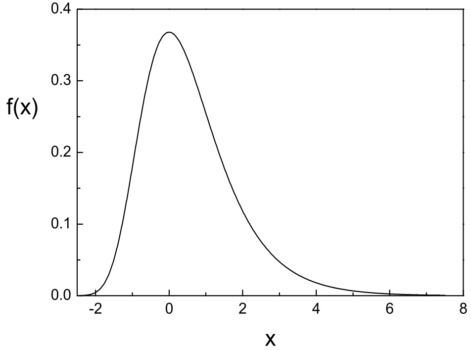
Fig. 3.22. Log-Weibull distribution.
