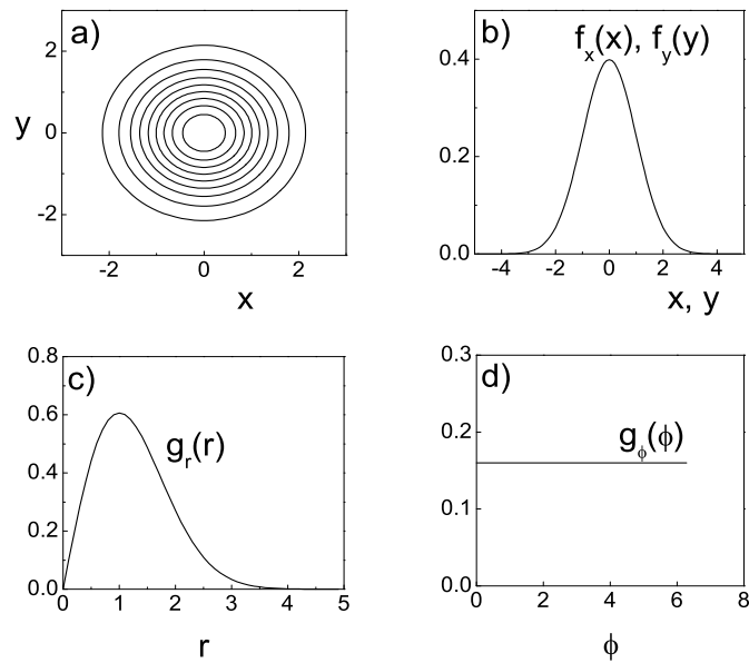
Fig. 3.13. Transformation of a two-dimensional normal distribution of cartesian coordinates into the distribution of polar coordinates.: (a) lines of constant probability; b) cartesian marginal distributions; c), d) marginal distributions of the polar coordinates.
