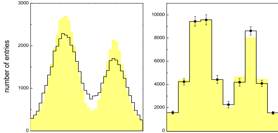
Fig. 9.5. Implicit regularization. Left hand: true (shadowed) and smeared histograms. Right hand: true (shadowed) and unfolded histograms without explicit regularization.
