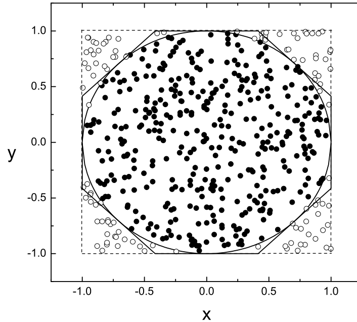
Fig. 5.12. Estimation of the number \pi .
