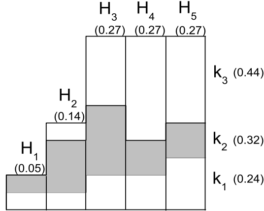
Fig. 6.1. Quantitative Venn diagramm. The areas indicate the probabilities for certain combinations of hypotheses H_i and discrete events of type k_j .
