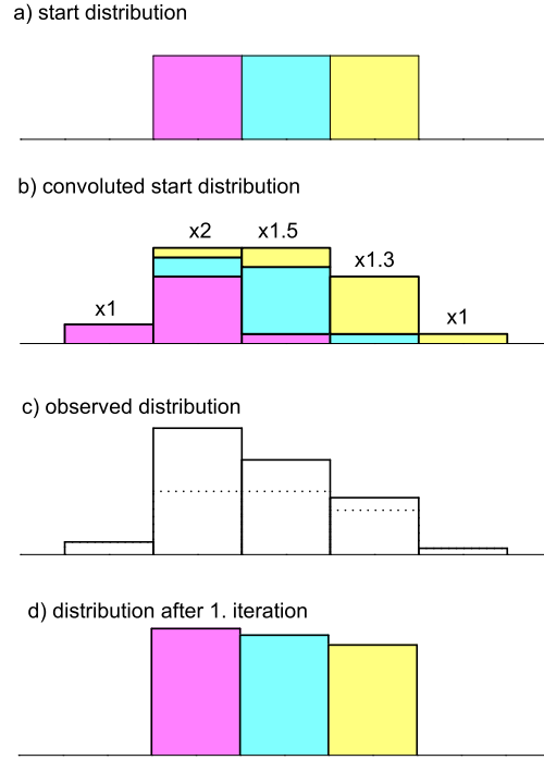
Fig. 9.6. Iterative deconvolution.
