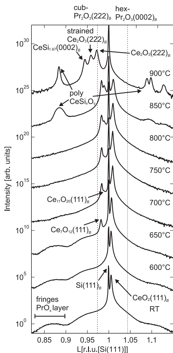
Fig. 9 Specular (00L) XRD scans close to the Si(111) B Bragg peak of the substrate. The samples are annealed at temperatures up to 900°C for 30 min. After each temperature step, the samples are cooled to RT and the measurements are performed. The as grown sample shows only the CeO 2 (111) peak next to the substrate. At temperatures above 600°C and 650°C peaks attributed to Ce 7 O 12 (111) and Ce 11 O 20 (111) appear, respectively. Thereafter, silicide and silicate peaks appear at temperatures above 800°C. The observed fringes correspond to the underlying praseodymia buffer layer. The Bragg peak of the buffer layer seems shifted to L values close to the cub-Pr 2 O 3 (222) B peak rather than the expected for hex-Pr 2 O 3 (0002) B peak (dashed lines). Therefore, an oxidation of the praseodymia layer during growth is assumed.
