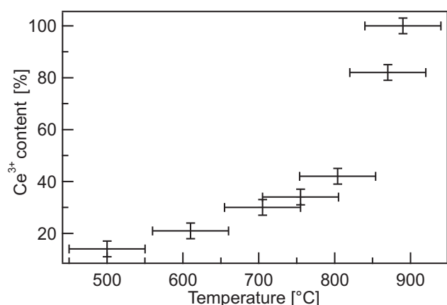
Fig. 3 Plot of the \text{Ce}^{3+} concentration as determined by the analysis of the Ce 3d spectra against the annealing temperature. The near surface region is continuously reduced with increasing temperature. After annealing at temperatures above 800^\circ\text{C} , the \text{Ce}^{3+} concentration increases drastically.
