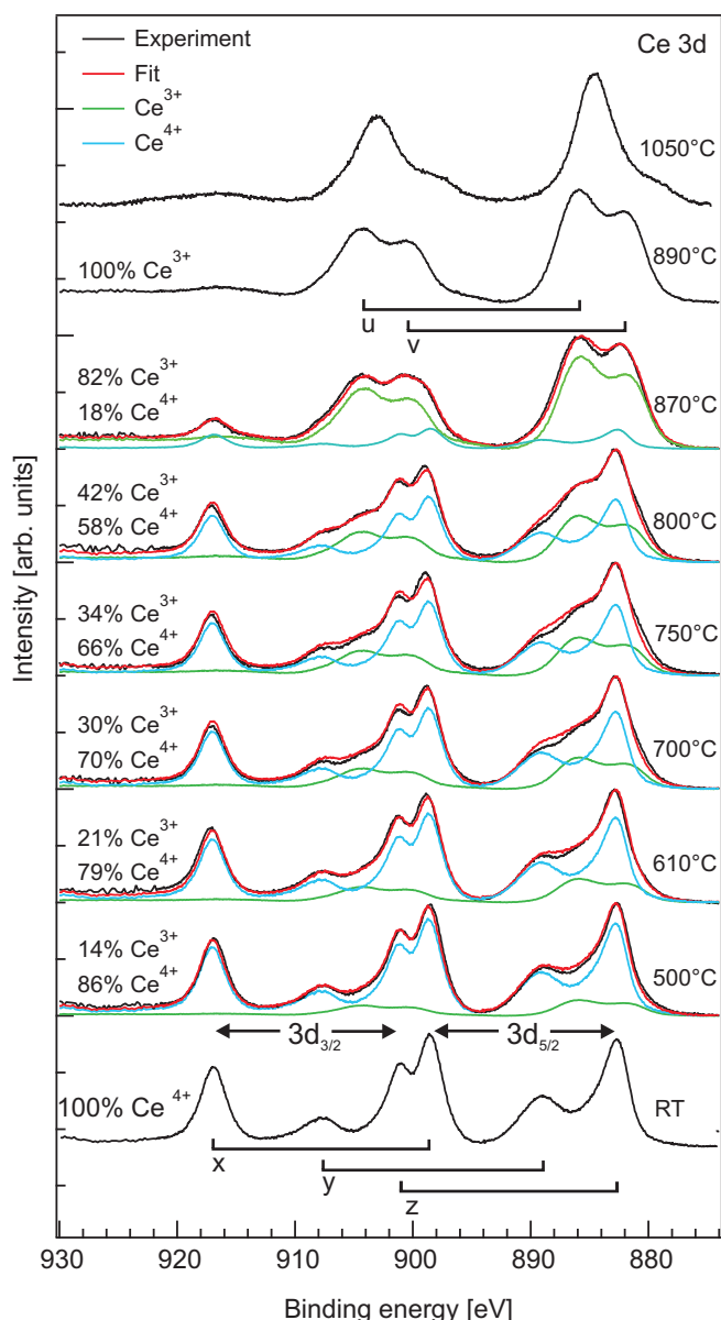
Fig. 2 XP spectra of the Ce 3d region. The area underneath the peaks is normalized to unity after a Shirley background is subtracted. The CeO 2 spectrum measured on the untreated sample consists of three peaks (x, y, z) in each 3d 5/2 and 3d 3/2 component. All cations have the Ce 4+ valence state. The surface near region is fully reduced to Ce 2 O 3 after annealing at 890°C where all cations have the Ce 3+ valence state. The spectrum consists of two peaks (u, v) in each 3d 5/2 and 3d 3/2 component. The determination of the Ce 3+ /Ce 4+ ratio of the intermediate states was done by fitting the spectra with a weighted linear combination of the CeO 2 and Ce 2 O 3 spectra. After annealing at 1050°C the peaks u and v shift \approx 1.2 eV and \approx 2.8 eV to lower binding energies due to silicide or silicate formation.
