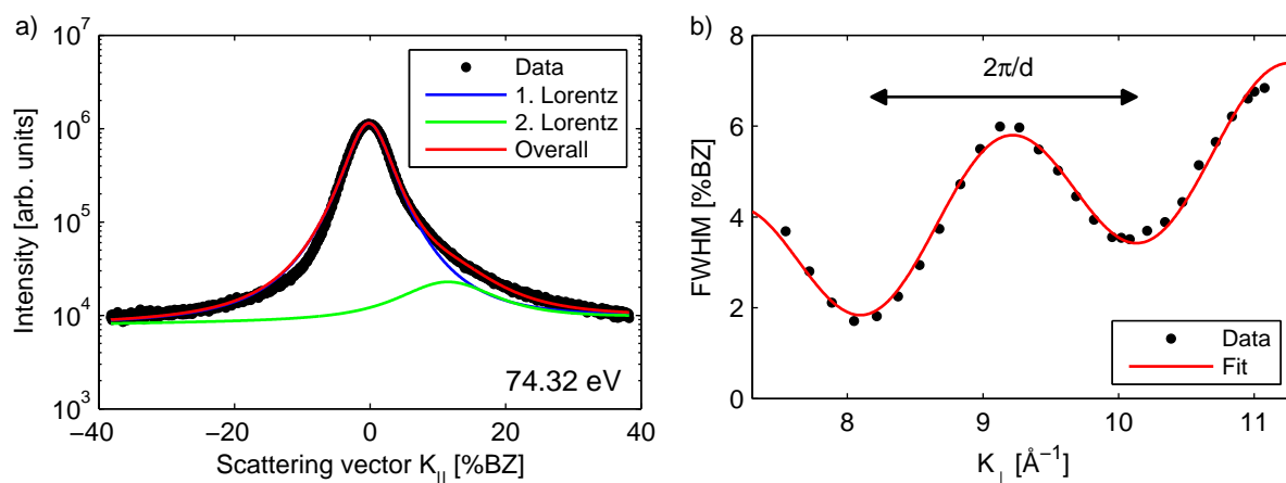
Fig. 7 (a) Cross section in the SPA-LEED pattern along the [11\bar{2}] direction after annealing at 500^\circ\text{C} for 30 min. The central peak (blue) and the shoulder (green) are fitted with Lorentzian functions. (b) FWHM of the central peak plotted against K_\perp after annealing at 500^\circ\text{C} for 30 min. The fit according to Eq. 1 is in good agreement with the experimental data.
