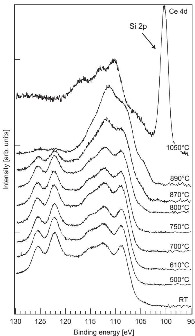
Fig. 4 XP spectra of the Ce 4d region normalized to the Ce 3d signal. After annealing at 1050^\circ\text{C} a strong Si 2p peak ( E_B = 100.3 eV) appears.
