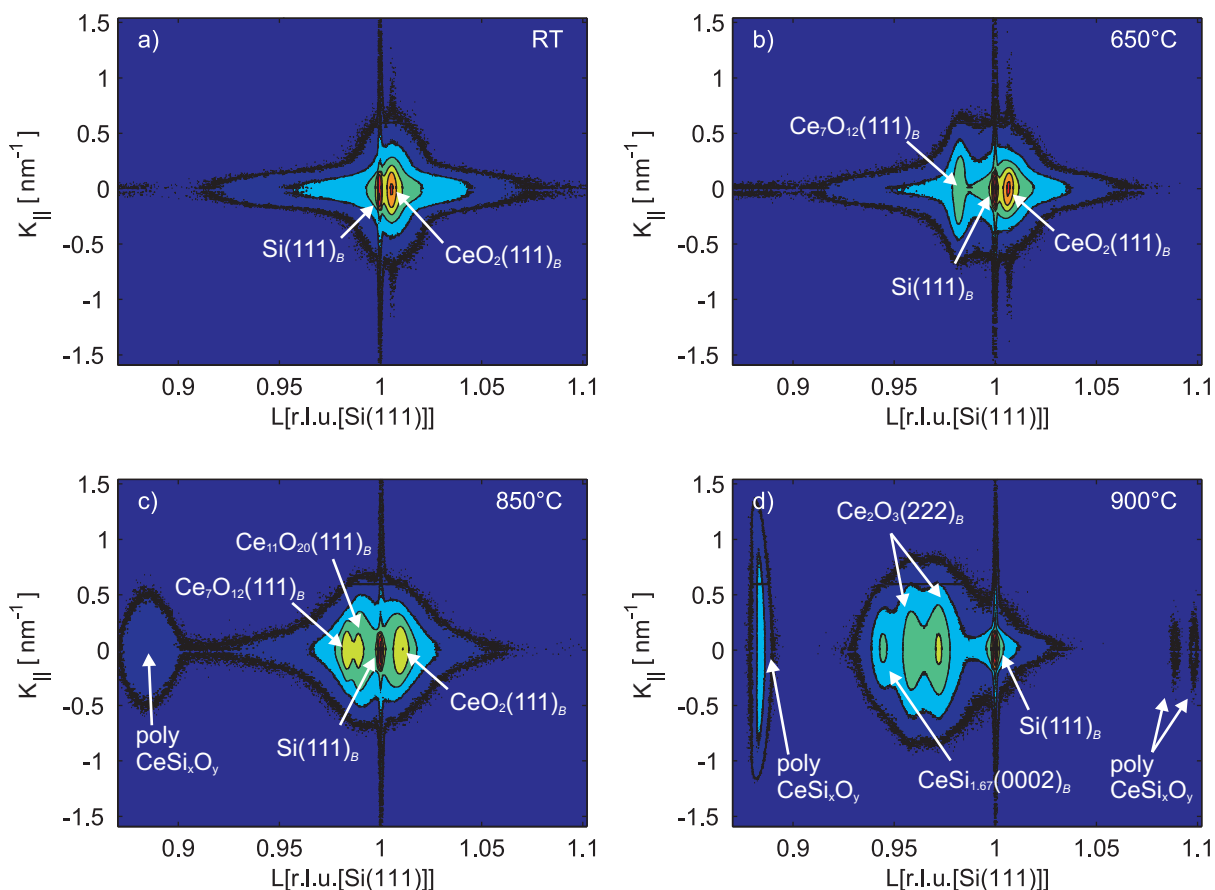
Fig. 8 Reciprocal space mappings close to the Si(111) Bragg peak obtained for annealing at different temperatures. The measurements are performed at RT. After annealing above 850°C, elongated features pointing to a polycrystalline structure appear at L = 0.89, 1.09, 1.10 .
