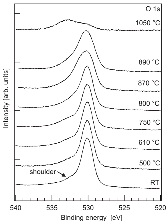
Fig. 5 XPS spectra of the O 1s peak ( E_B = 530.2 eV) exhibiting a weak shoulder at E_B \approx 532 eV. The spectra are normalized to the Ce 3d signal. The FWHM of the O 1s peak increases after annealing above 800 °C. The intensity of the O 1s peak is drastically reduced after annealing at 1050 °C and the shoulder shifts to higher binding energies indicating Si-O bonds.
