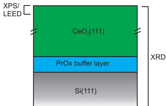
Fig. 1 Schematic drawing of the investigated system. XPS and LEED are used to probe the near surface region while changes of the entire structure are studied by XRD.
