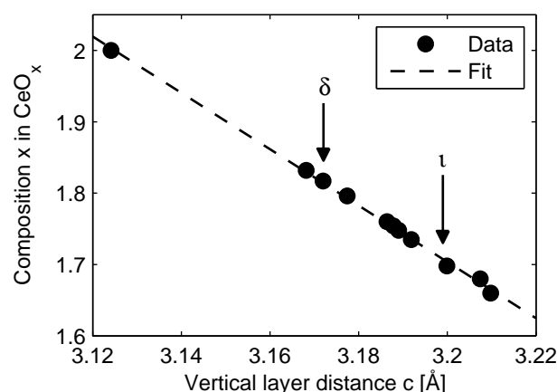
Fig. 10 Composition of the film expressed as the stoichiometry parameters x plotted against the vertical layer distance c according to the pseudo-cubic lattice parameters given by Ref. 20,50 .
