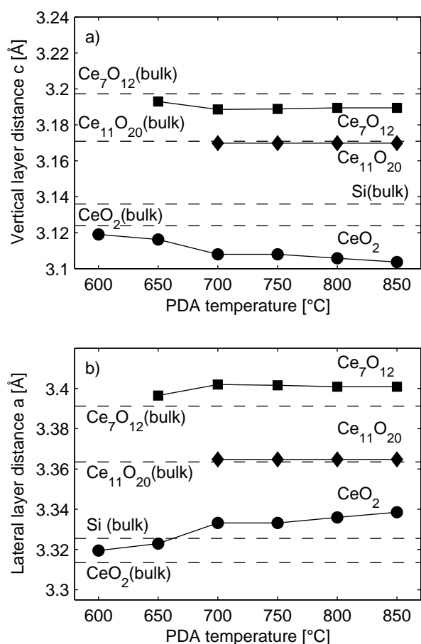
Fig. 11 (a) Vertical layer distance of the appearing ceria phases plotted against the PDA temperature. The stoichiometry of the different phases was determined by their pseudo-cubic lattice constant from Eq. 2. (b) Lateral layer distance determined from Eq. 3. The layer distances of the \text{CeO}_2 and \text{Ce}_7\text{O}_{12} differ from the bulk value indicating strained films while the \text{Ce}_{11}\text{O}_{20} phase is fully relaxed.
