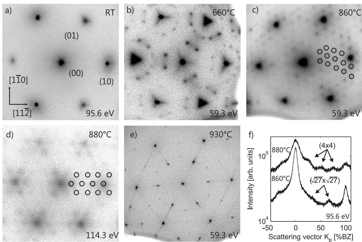
Fig. 6 Two dimensional SPA-LEED pattern of the appearing structures close to Bragg conditions (in-phase) of \text{CeO}_2(111) . (a) The (1 \times 1) structure of the sample stays unchanged at low and moderate temperatures. (b) At a PDA temperature of 660^\circ\text{C} a (\sqrt{7} \times \sqrt{7})\text{R}19.1^\circ superstructure attributed to the \iota -phase ( \text{Ce}_7\text{O}_{12} ) appears. (c) In the narrow temperature region of 850^\circ\text{C} - 870^\circ\text{C} a (\sqrt{27} \times \sqrt{27})\text{R}30^\circ structure forms. (d) A weak (4 \times 4) structure assigned to the bixbyite phase of \text{Ce}_2\text{O}_3 appears at PDA temperatures of 880^\circ\text{C} - 890^\circ\text{C} . (e) After annealing above 900^\circ\text{C} , a sharp (2 \times 1) pattern superimposed with a (\sqrt{3} \times \sqrt{3})\text{R}30^\circ structure appears which can be assigned to cerium silicide. (f) Cross section along the [112] direction. The (\sqrt{27} \times \sqrt{27})\text{R}30^\circ and the (4 \times 4) structures show two and three peaks between the fundamental diffraction spots, respectively.
