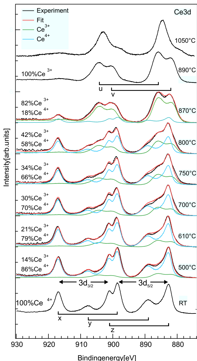
Fig. 2 XP spectra of the Ce 3d region. The area underneath the peaks is normalized to unity after a Shirley background is subtracted. The \text{CeO}_2 spectrum measured on the untreated sample consists of three peaks (x, y, z) in each 3d_{5/2} and 3d_{3/2} component. All cations have the \text{Ce}^{4+} valence state. The surface near region is fully reduced to \text{Ce}_2\text{O}_3 after annealing at 890^\circ\text{C} where all cations have the \text{Ce}^{3+} valence state. The spectrum consists of two peaks (u, v) in each 3d_{5/2} and 3d_{3/2} component. The determination of the \text{Ce}^{3+}/\text{Ce}^{4+} ratio of the intermediate states was done by fitting the spectra with a weighted linear combination of the \text{CeO}_2 and \text{Ce}_2\text{O}_3 spectra. After annealing at 1050^\circ\text{C} the peaks u and v shift \approx 1.2 eV and \approx 2.8 eV to lower binding energies due to silicide or silicate formation.
