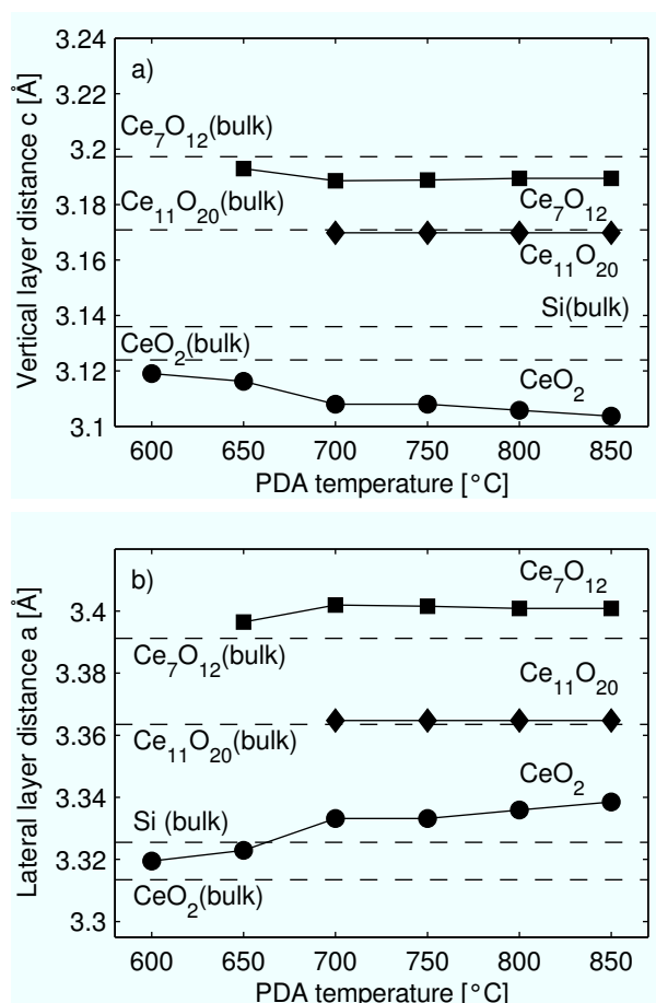
Fig. 11 (a) Vertical layer distance of the appearing ceria phases plotted against the PDA temperature. The stoichiometry of the different phases was determined by their pseudo-cubic lattice constant from Eq. 2. (b) Lateral layer distance determined from Eq. 3. The layer distances of the \text{CeO}_2 and \text{Ce}_7\text{O}_{12} differ from the bulk value indicating strained films while the \text{Ce}_{11}\text{O}_{20} phase is fully relaxed.
