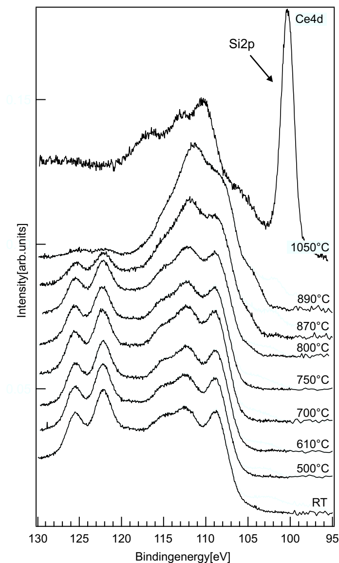
Fig. 4 XP spectra of the Ce 4d region normalized to the Ce 3d signal. After annealing at 1050^\circ\text{C} a strong Si 2p peak ( E_B = 100.3 eV) appears.
