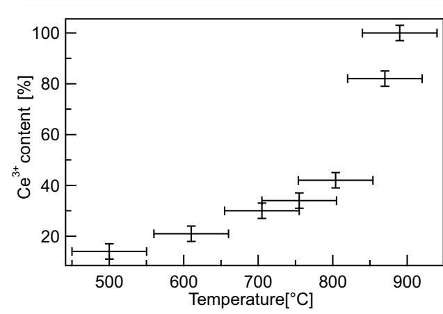
Fig. 3 Plot of the \text{Ce}^{3+} concentration as determined by the analysis of the Ce 3d spectra against the annealing temperature. The near surface region is continuously reduced with increasing temperature. After annealing at temperatures above 800^\circ\text{C} , the \text{Ce}^{3+} concentration increases drastically.
