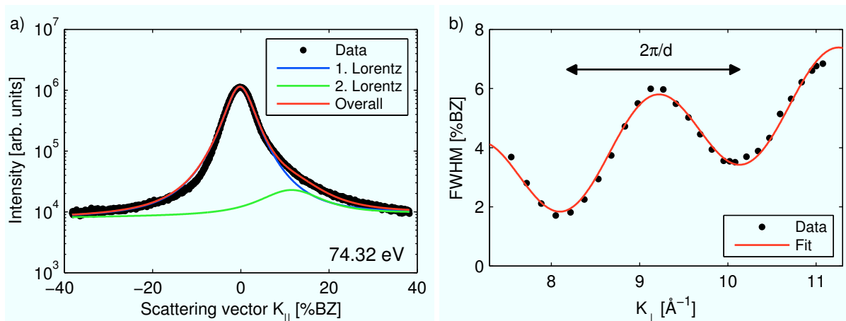
Fig. 7 (a) Cross section in the SPA-LEED pattern along the [11\bar{2}] direction after annealing at 500^\circ\text{C} for 30 min. The central peak (blue) and the shoulder (green) are fitted with Lorentzian functions. (b) FWHM of the central peak plotted against K_\perp after annealing at 500^\circ\text{C} for 30 min. The fit according to Eq. 1 is in good agreement with the experimental data.
