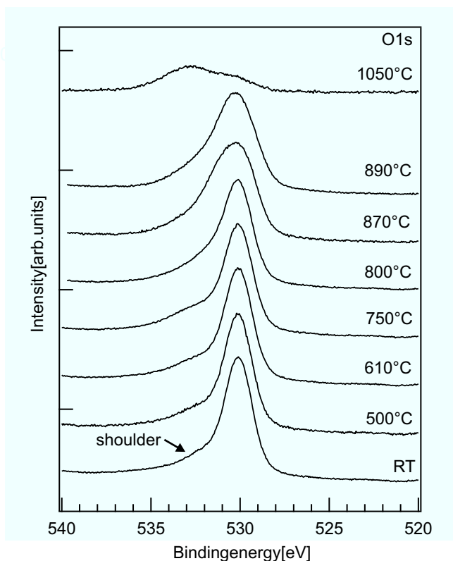
Fig. 5 XPS spectra of the O 1s peak ( E_B = 530.2 eV) exhibiting a weak shoulder at E_B \approx 532 eV. The spectra are normalized to the Ce 3d signal. The FWHM of the O 1s peak increases after annealing above 800°C. The intensity of the O 1s peak is drastically reduced after annealing at 1050°C and the shoulder shifts to higher binding energies indicating Si-O bonds.
