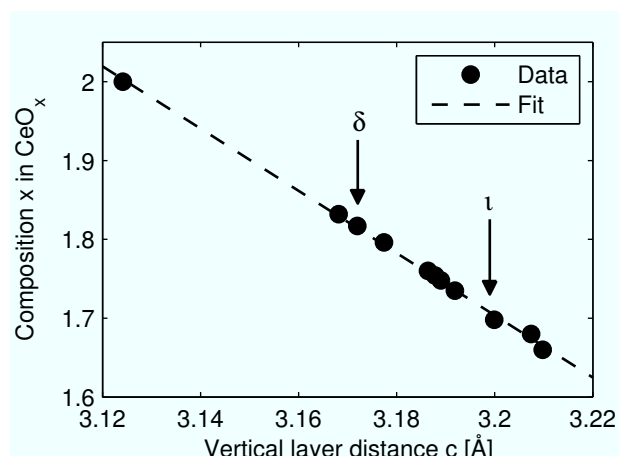
Fig. 10 Composition of the film expressed as the stoichiometry parameters x plotted against the vertical layer distance c according to the pseudo-cubic lattice parameters given by Ref. 20,50 .
