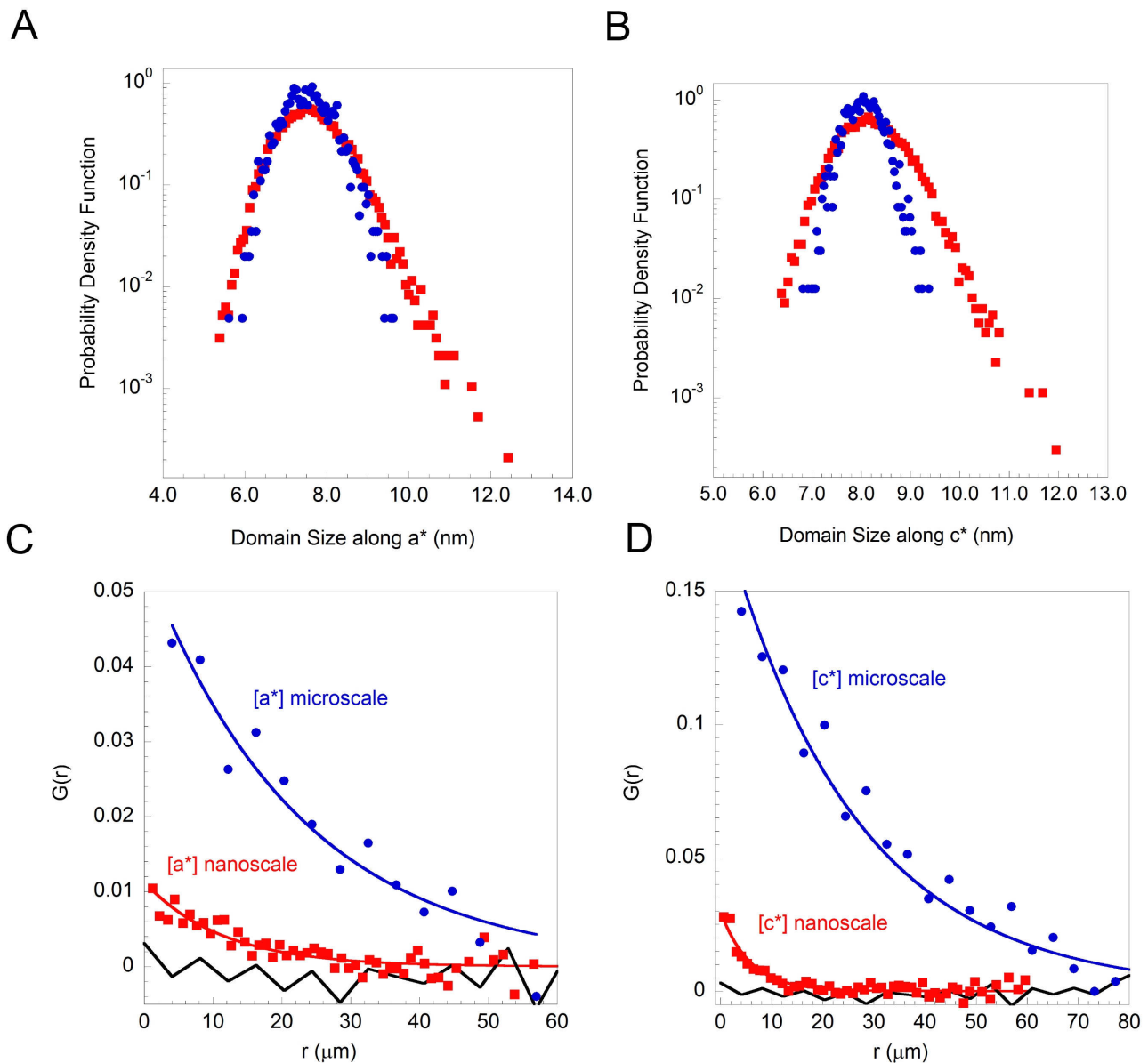
Figure 4 | Probability density function of the domain size along a -axis (A) and along c -axis (B) obtained by the microbeam (filled circles) and the nanobeam (filled squares) measurements. Radial correlation function G(r) calculated on domain size map along a -axis (C) and c -axis (D). The blue circles and the red filled squares correspond to the \mu\text{XRD} and \text{nXRD} measurements. A comparison between the G(r) behaviors is shown.
