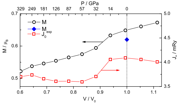
FIG. 4 (color online). Dependence of the calculated magnetic moment M (circle) and the effective exchange interaction parameter J_0 (square) on the unit cell volume V normalized with respect to the equilibrium volume V_0 of ferromagnetic fcc Ni. The experimental value of the magnetic moment of Ni at zero pressure [38] is shown for comparison (diamond).
