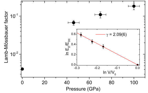
FIG. 5 (color online). Pressure dependence of the Lamb-Mössbauer factor. The inset shows the logarithm of the Debye energy as a function of the logarithm of the volume. The linear fit shown by the line gives the Grüneisen parameter \gamma .
