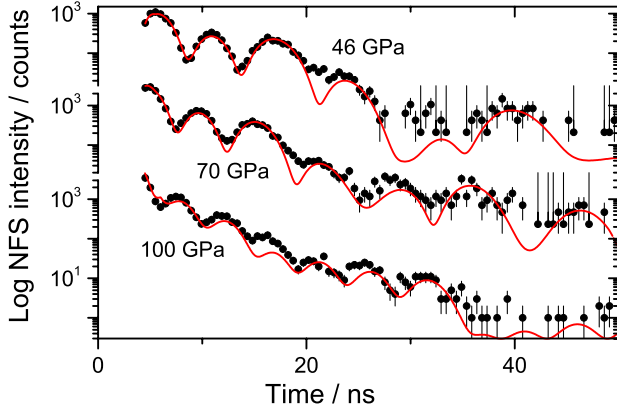
FIG. 2 (color online). Time evolution of the nuclear forward scattering for Ni measured perpendicular to the DAC axis at room temperature. The solid lines show the fit according to the model described in the text.
