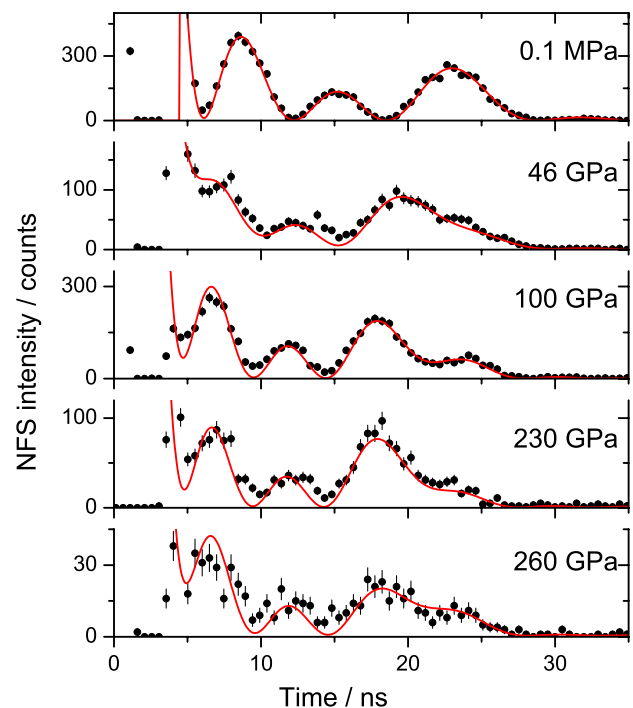
FIG. 1 (color online). Time evolution of the nuclear forward scattering for Ni measured along the DAC axis at room temperature. The solid lines show the fit according to the model described in the text.
