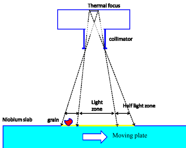
Figure 2: Set-up arrangement for lateral sample scanning.
