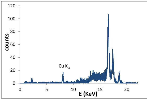
Figure 1: XRF Spectrum of Nb sample with Cu \mu\text{g} impurity.
