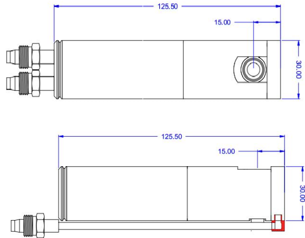
Figure 5: Linear dimensions of X-ray tube, expressed in mm. Courtesy of ProtoXRD.
