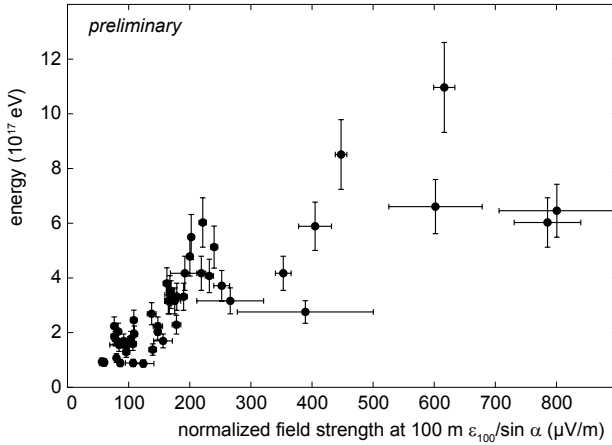
Figure 6: Correlation between the radio field strength at 100 m corrected for the geomagnetic effect and the energy reconstructed with the air-Cherenkov measurements. The given values for the field strength are based on a preliminary calibration.
