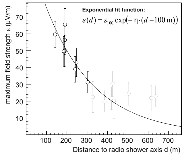
Figure 5: Lateral distribution of the radio amplitude (= maximum field strength) for the example event shown in Fig. 2.
