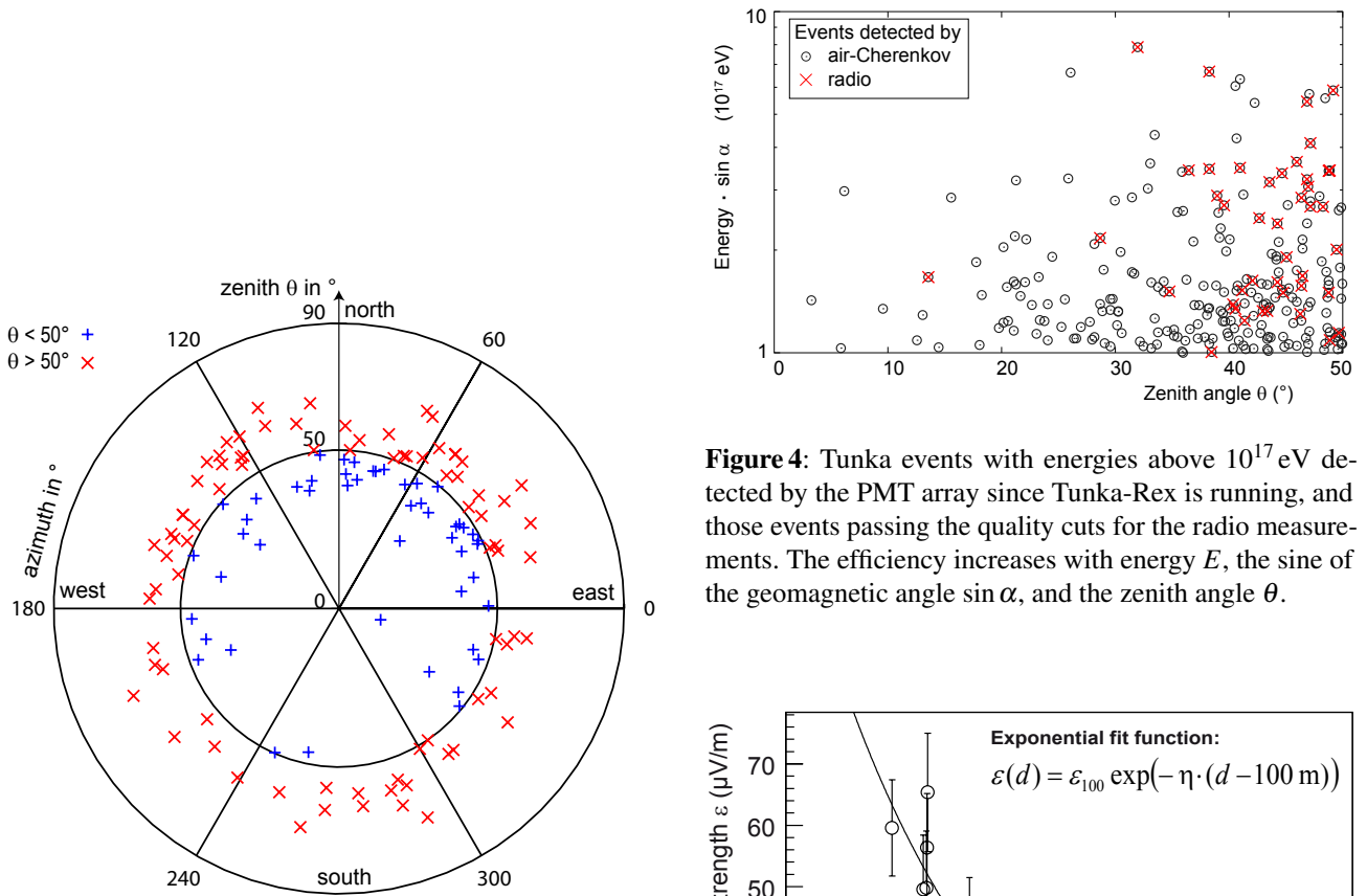
Figure 3: Arrival directions of the Tunka-Rex events passing the quality cuts. Due to the geomagnetic effect, the radio signal is expected to be on average stronger for events coming from North, which explains the asymmetry in the detection efficiency: 89 of the 131 events are in the northern half of the plot, and 42 in the southern half.
