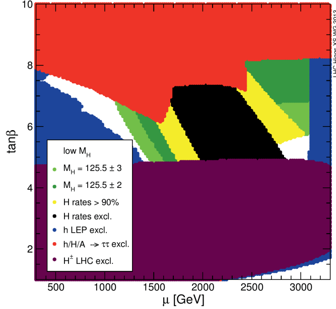
Figure 132: Experimentally favored and excluded regions in the \mu - \tan\beta plane in the low\text{-}M_H scenario. The green shades indicate the region where M_H = 125.5 \pm 2 (3) GeV. The yellow and black areas also have M_H = 125.5 \pm 3 GeV, where the yellow area additionally satisfies the requirement that the rates for the gg \rightarrow H , H \rightarrow \gamma\gamma and H \rightarrow ZZ^* channels, are at least at 90% of their SM value for the same Higgs mass. The black region indicates where the rates for H decay to gauge bosons become too high, such that these points are excluded by HIGGSBOUNDS. As before, the blue area is excluded by LEP Higgs searches, whereas the solid red is excluded from LHC searches for the neutral MSSM Higgs bosons, h , H and A in the \tau^+\tau^- decay channel. The purple region is excluded by charged Higgs boson searches at the LHC. The white area at very large values of \mu and low \tan\beta is unphysical, i.e. this parameter region is theoretically inaccessible.
