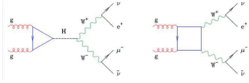
Figure 115: Diagrams for the gg \rightarrow H \rightarrow WW \rightarrow lv_l lv_l process (left) and the continuum gg \rightarrow WW \rightarrow lv_l lv_l process (right).
