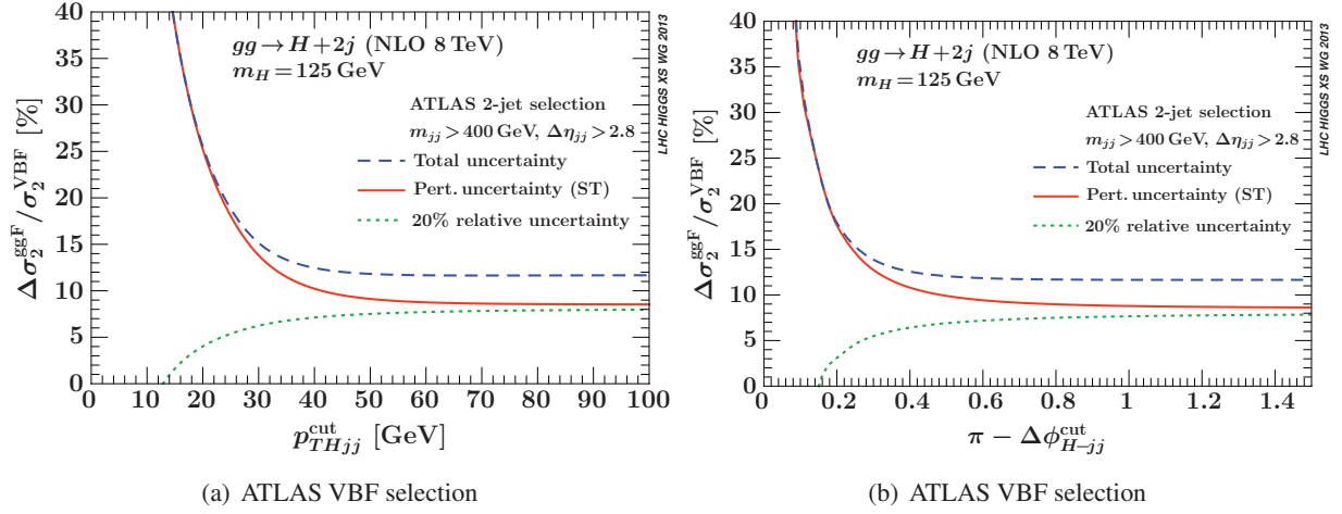
Fig. 66: Theoretical uncertainties of the ggF contribution relative to the VBF cross section as function of p_{THjj}^{\text{cut}} (left) and \Delta\phi_{Hjj}^{\text{cut}} (right) for the ATLAS VBF selection.
