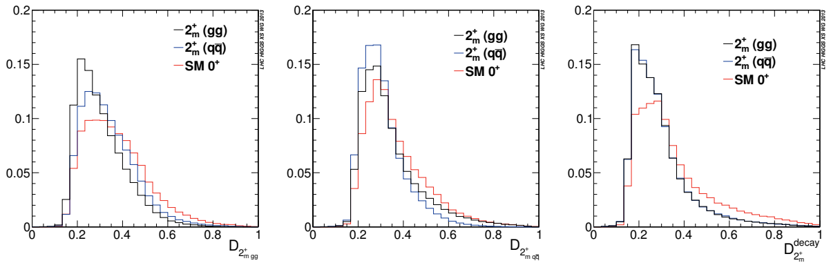
Figure 92: Distribution of the discriminants D_{2m}^{+} (left), D_{2m}^{+} (middle), D_{2m}^{decay} (right) evaluated with three different samples: SM Higgs boson, spin-two produced through gluon-gluon fusion and produced through q\bar{q} annihilation.
