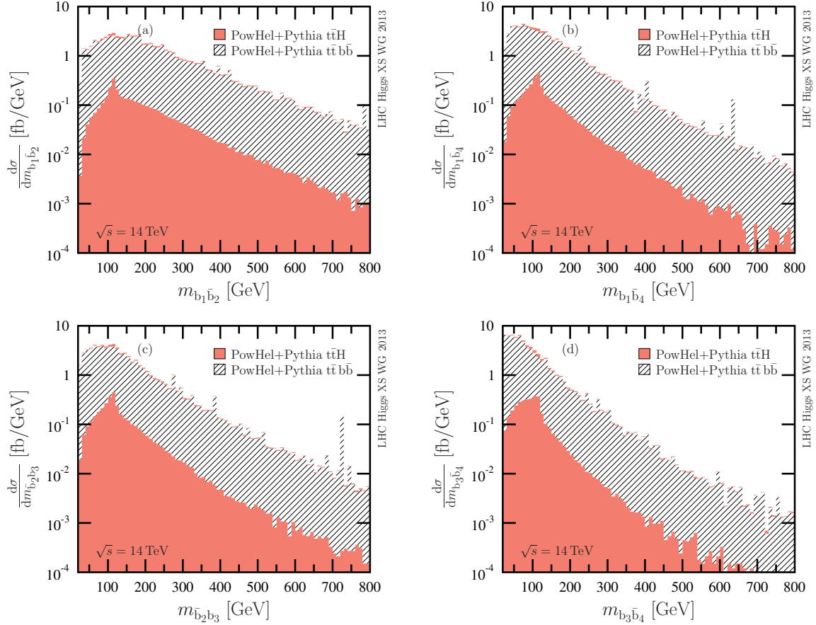
Fig. 52: Invariant mass of the four possible b -jet pairs with one b - and one \bar{b} -tagged jet in the pairs. The t\bar{t}H and the t\bar{t}b\bar{b} distributions after POWHEG+PYTHIA are shown by pink and shaded black histograms, respectively. Peaks around the Higgs mass are visible in the t\bar{t}H distributions.
