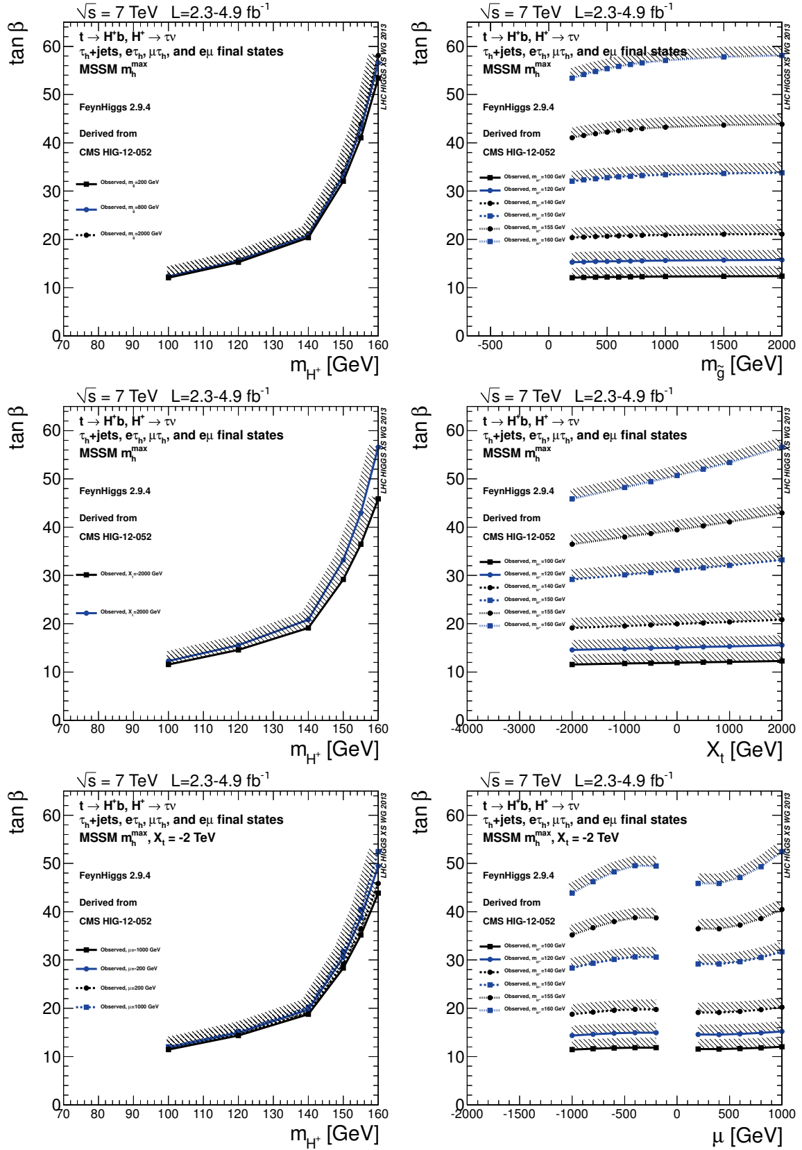
Figure 138: The effect of varying M_{\tilde{g}} on the experimentally excluded region in the m_{H^+}^{\max} scenario (top left and right), the effect of varying X_t (middle plots), and the effect of varying the \mu parameter with X_t = -2 TeV (bottom plots).
