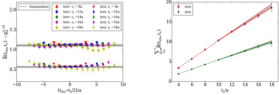
Figure 2: Left: \tilde{R}(t_{\text{ins}}, t_s) for the isovector (squares) and connected isoscalar (circles) axial charge. The blue bands show the plateau-value for t_s/a = 12 . The gray bands are the results extracted by fitting to the slope of the summed ratio as shown in the right panel. A total of 1200 measurements were used for each t_s .
