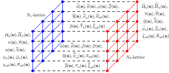
Figure 6: Schematic sketch of the lattice construction of two-dimensional Q = 8 quiver gauge theory. The lattice variables \{\mathcal{U}_a(\mathbf{n}), \bar{\mathcal{U}}_a(\mathbf{n}), \pi(\mathbf{n}), \bar{\pi}(\mathbf{n}), \eta(\mathbf{n}), \psi_a(\mathbf{n}), \chi_{ab}(\mathbf{n}), \bar{\lambda}(\mathbf{n}), \bar{w}_a(\mathbf{n}), \bar{\sigma}_{ab}(\mathbf{n})\} live on the two-dimensional N_1 -lattice spacetime and \{\hat{\mathcal{U}}_a(\mathbf{n}), \hat{\bar{\mathcal{U}}}_a(\mathbf{n}), \hat{\pi}(\mathbf{n}), \hat{\bar{\pi}}(\mathbf{n}), \hat{\eta}(\mathbf{n}), \hat{\psi}_a(\mathbf{n}), \hat{\chi}_{ab}(\mathbf{n}), \hat{\bar{\lambda}}(\mathbf{n}), \hat{\bar{w}}_a(\mathbf{n}), \hat{\bar{\sigma}}_{ab}(\mathbf{n})\} live on the two-dimensional N_2 -lattice spacetime. The matter fields \{\phi(\mathbf{n}), \hat{\phi}(\mathbf{n}), \bar{\phi}(\mathbf{n}), \bar{\phi}(\mathbf{n}), \bar{\eta}(\mathbf{n}), \hat{\psi}_a(\mathbf{n}), \bar{\kappa}_{ab}(\mathbf{n}), \bar{\rho}_a(\mathbf{n}), \bar{\tau}_a(\mathbf{n}), \hat{\xi}_{ab}(\mathbf{n})\} and \{\hat{\phi}(\mathbf{n}), \hat{\phi}(\mathbf{n}), \varphi(\mathbf{n}), \bar{\varphi}(\mathbf{n}), \hat{\eta}(\mathbf{n}), \bar{\psi}_a(\mathbf{n}), \hat{\kappa}_{ab}(\mathbf{n}), \bar{\rho}_a(\mathbf{n}), \bar{\tau}_a(\mathbf{n}), \bar{\xi}_{ab}(\mathbf{n})\} live on the links connecting the two lattices.
