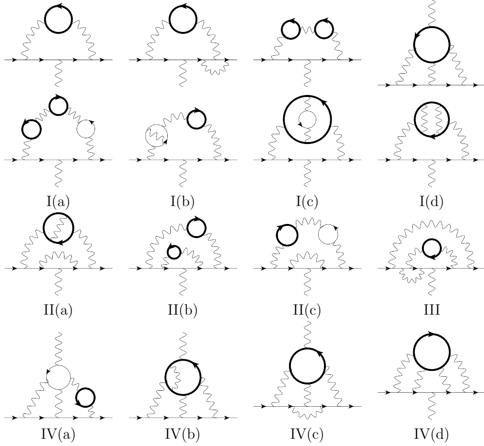
Figure 1: Sample Feynman diagrams contributing to the electron and muon (g - 2) containing a heavy lepton at two, three and four loops. Thin and thick solid lines represent light and heavy leptons, respectively, and wavy lines denote photons. The symbols below the four-loop diagrams label the individual diagram classes and are taken over from Refs. [7, 22].
