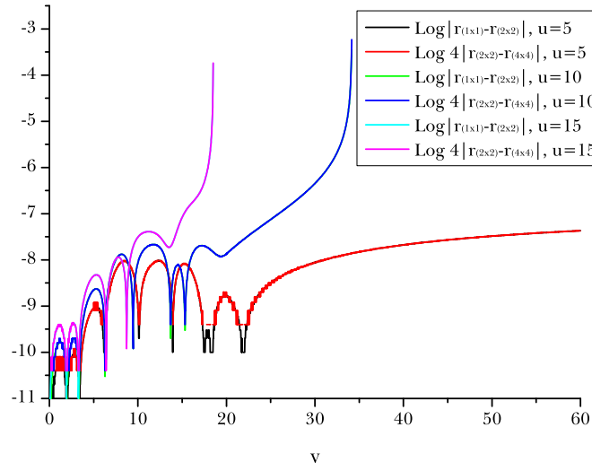
Figure 9. Convergence test for \kappa = 0.05 , A = 7000 , m^2 = 0.05 .
