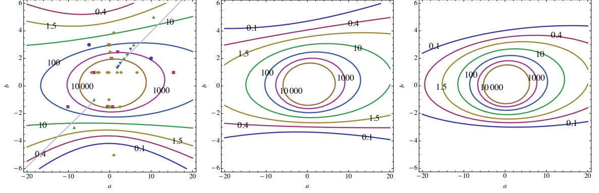
Figure 8: Analytic results for the gaugino focus point scale (in units of TeV) in the GNMSSM for \lambda = 1.5 (at the GUT scale) and \tan\beta = 2, 3, 10 from left to right. The contours do not change much for larger \tan\beta . The points and line shown are the same as shown in Fig. 1.
