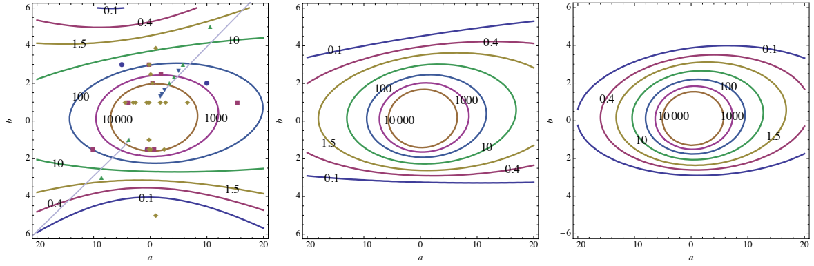
Figure 1: Analytic results for the gaugino focus point scale contours (in units of TeV) in the MSSM for \tan \beta = 2, 3, 10 from left to right. The points and the gray line correspond to specific models with non-universal gaugino masses; see text for details. The contours do not change much for larger \tan \beta .
