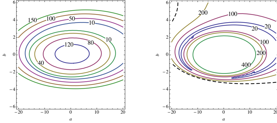
Figure 2: Analytic results for minimal fine tuning in the MSSM in the limit \tan \beta \rightarrow \infty before (left) and after (right) the Higgs mass cut. The region below the black dashed line corresponds to very large scalar masses, m_0 > 5 TeV.
