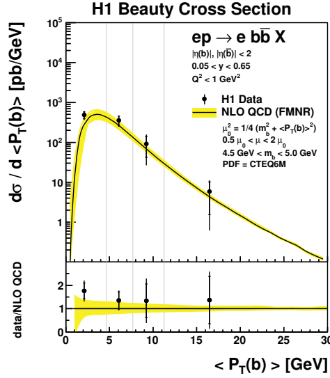
Figure 1. Differential beauty cross section d\sigma/d\langle P_T(b) \rangle shown as a function of the quadratically averaged transverse momentum of the beauty quarks \langle P_T(b) \rangle (upper part). The data are represented by points with the inner vertical error bars representing the statistical errors and the full error bars representing the total uncertainty. The vertical grey lines indicate the bin boundaries in \langle P_T(b) \rangle of each data point and the points are shown at the bin centre positions. The data are compared to the FMNR NLO QCD calculation (solid line) with the uncertainty represented as a shaded band. In the lower part, the ratio of the measured cross section to the calculated NLO QCD prediction is shown.
