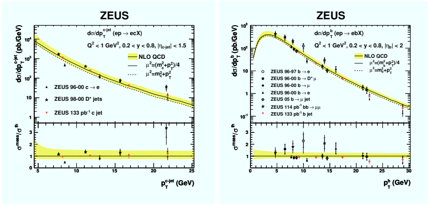
Figure 5. Charm (left) and beauty (right) cross section as a function of the c -jet and of the b -jet, respectively. The data is represented by black points and the NLO predictions by coloured bands. The vertical error bars represent the total uncertainty, with the inner error bars depicting the statistical uncertainty.
