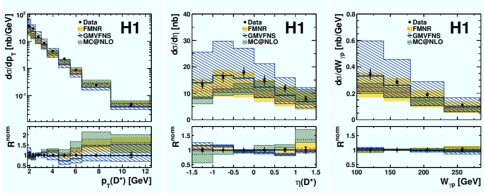
Figure 2. Cross section as a function of p_T(D^*) (left), \eta(D^*) (middle) and W_{\gamma p} (right). The data is represented by black points and the NLO predictions by coloured bands. The vertical error bars represent the total uncertainty, with the inner error bars depicting the statistical uncertainty.
