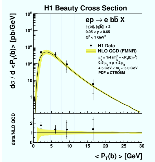
Figure 1. Differential beauty cross section d\sigma/d\langle P_T(b) \rangle shown as a function of the quadratically averaged transverse momentum of the beauty quarks \langle P_T(b) \rangle (upper part). The data are represented by points with the inner vertical error bars representing the statistical errors and the full error bars representing the total uncertainty. The vertical grey lines indicate the bin boundaries in \langle P_T(b) \rangle of each data point and the points are shown at the bin centre positions. The data are compared to the FMNR NLO QCD calculation (solid line) with the uncertainty represented as a shaded band. In the lower part, the ration of the measured cross section to the calculated NLO QCD prediction is shown.
