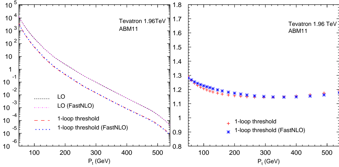
Figure 1: LO results and 1-loop threshold corrections \sigma^{(1)} for the transverse momentum distribution of the jet (left) and the corresponding K^{(1)} (right) at Tevatron.
