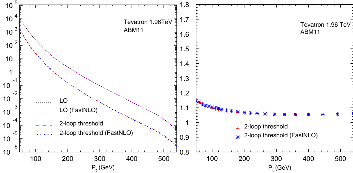
Figure 2: LO results and 2-loop threshold corrections \sigma^{(2)} for the transverse momentum distribution of the jet (left) and the corresponding K^{(2)} (right) at Tevatron.
