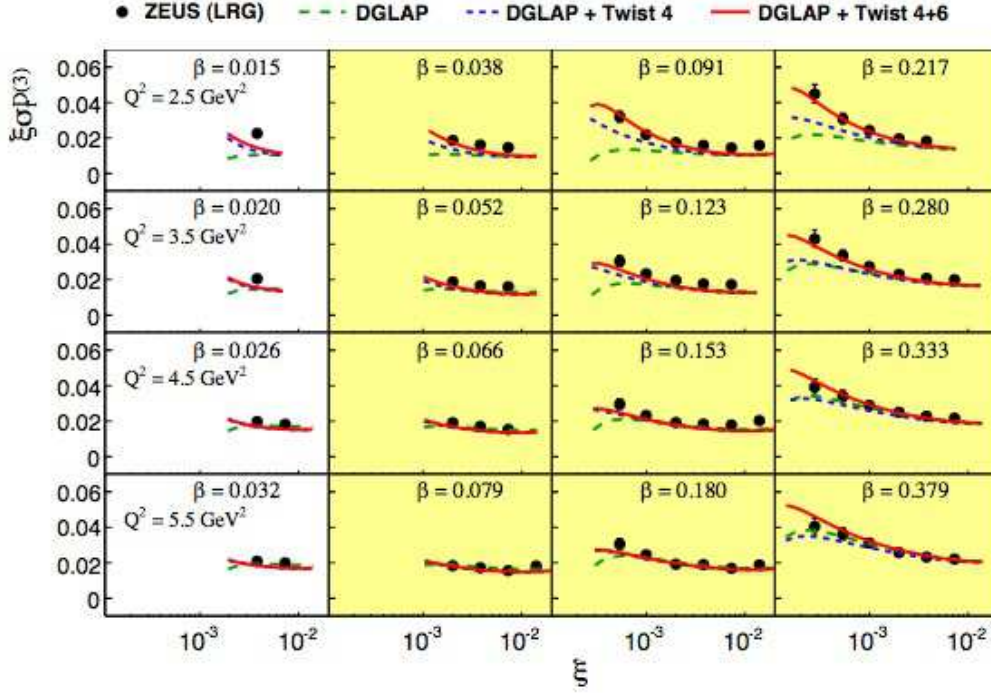
Figure 3: ZEUS diffractive cross section data compared to DGLAP predictions without and with twist 4 and 6 effects from the saturation model.
