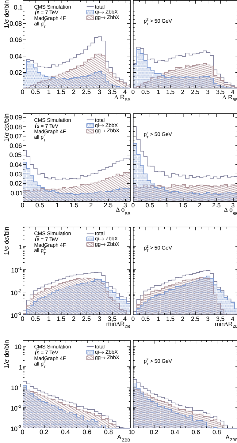
Figure 2: Distribution of \Delta R_{BB} (first row), \Delta \phi_{BB} (second row), \min \Delta R_{ZB} (third row), and A_{ZBB} (fourth row) as predicted by MADGRAPH in the four-flavour scheme, in the nonboosted (left) and boosted (right) regions of the Z transverse momentum. The component from gg \rightarrow ZbbX is represented by the hatched histogram, while the contribution from q\bar{q} \rightarrow ZbbX subprocesses (where i = q, g ) is represented by the shaded histogram. The unshaded histogram corresponds to the sum of the two components.
