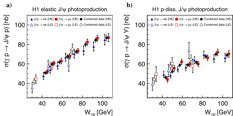
Fig. 5 Elastic and proton-dissociative J/\psi photoproduction cross sections as a function of W_{\gamma p} as obtained from the analysis of J/\psi \rightarrow e^+ e^- (triangles) and J/\psi \rightarrow \mu^+ \mu^- (squares) and by the combination of these two independent measurements (circles). The filled and open symbols refer to the results from the HE and LE data sets, respectively. The error bars of the independent measurements correspond to the sta-
