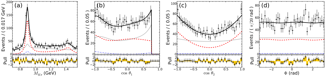
FIG. 5: Projections onto the observables (a) M_{K\pi} , (b) \cos \theta_1 , (c) \cos \theta_2 , and (d) \Phi for B^0 \rightarrow \phi(K^+\pi^-)^* and \bar{B}^0 \rightarrow \phi(K^-\pi^+)^* combined. The data distributions are shown by black markers with error bars whereas the overall fit function, combinatorial background, signal and peaking background are shown with solid black, dotted black, dashed red and dash-dotted blue curves, respectively. For each projection, the data points and fit projections are shown after a signal-enhancing selection (see text) on M_{bc} , \Delta E , M_{KK} and C'_{NB} shown in Fig. 4.
