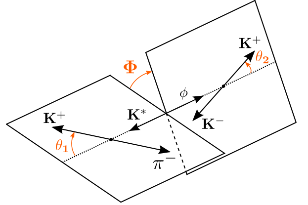
FIG. 2: Definition of the three helicity angles given in the rest frame of the parent particles for the B^0 \rightarrow \phi K^* decay.
