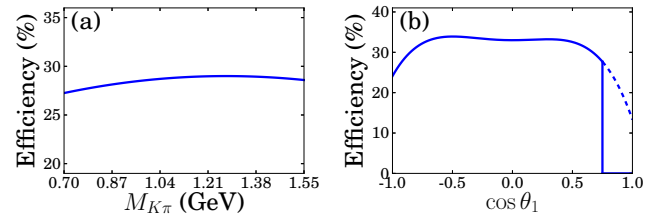
FIG. 3: Efficiency as a function of (a) M_{K\pi} and (b) \cos\theta_1 . In (b) the dashed line indicates the \cos\theta_1 region excluded from the analysis.
