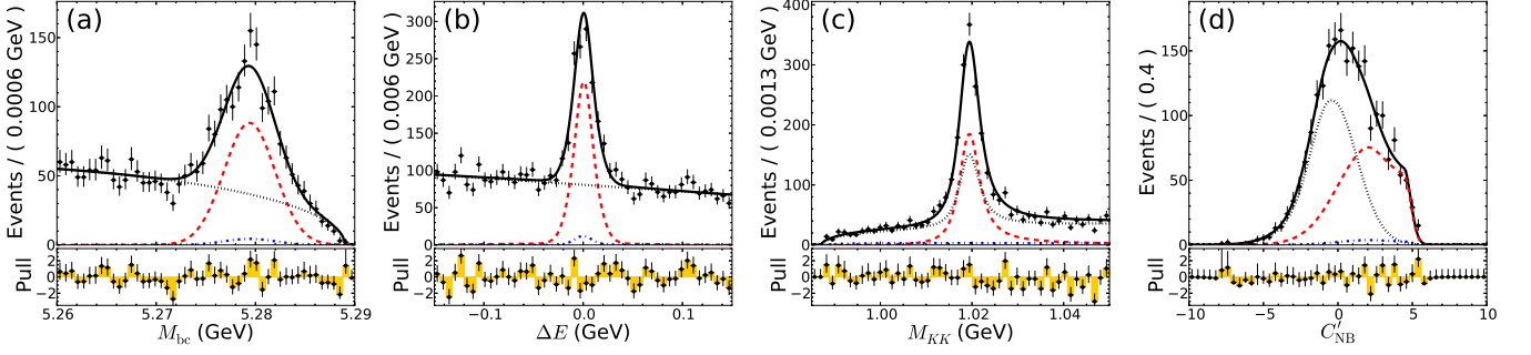
FIG. 4: Projections onto the observable (a) M_{bc} , (b) \Delta E , (c) M_{KK} , and (d) C'_{NB} for B^0 \rightarrow \phi(K^+\pi^-)^* and \bar{B}^0 \rightarrow \phi(K^-\pi^+)^* combined. The data distributions are shown by black markers with error bars whereas the overall fit function, combinatorial background, signal and peaking background are shown with solid black, dotted black, dashed red and dash-dotted blue curves, respectively. For each projection, the data points and fit projections are shown after a signal-enhancing selection (see text) on the other three observables; e.g., in (a) a requirement on (b),(c) and (d) is applied.
