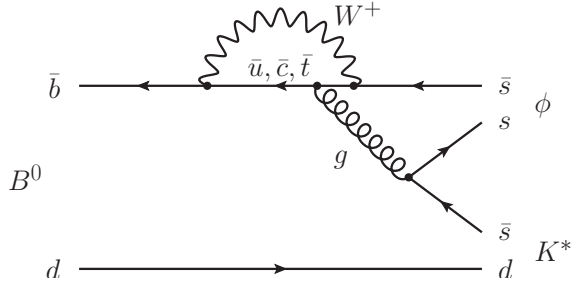
FIG. 1: Penguin diagram of the decay B^0 \rightarrow \phi K^* .
