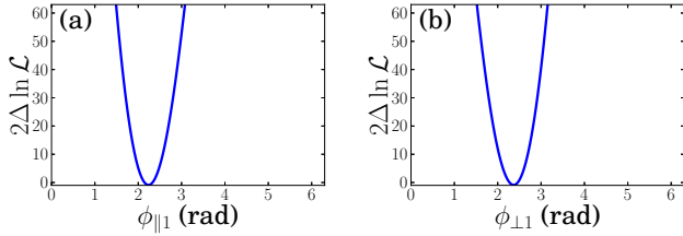
FIG. 6: Scan of the negative log likelihood as function of (a) \phi_{\parallel 1} and (b) \phi_{\perp 1} . One single discrete solution is found for each of the two phases.
