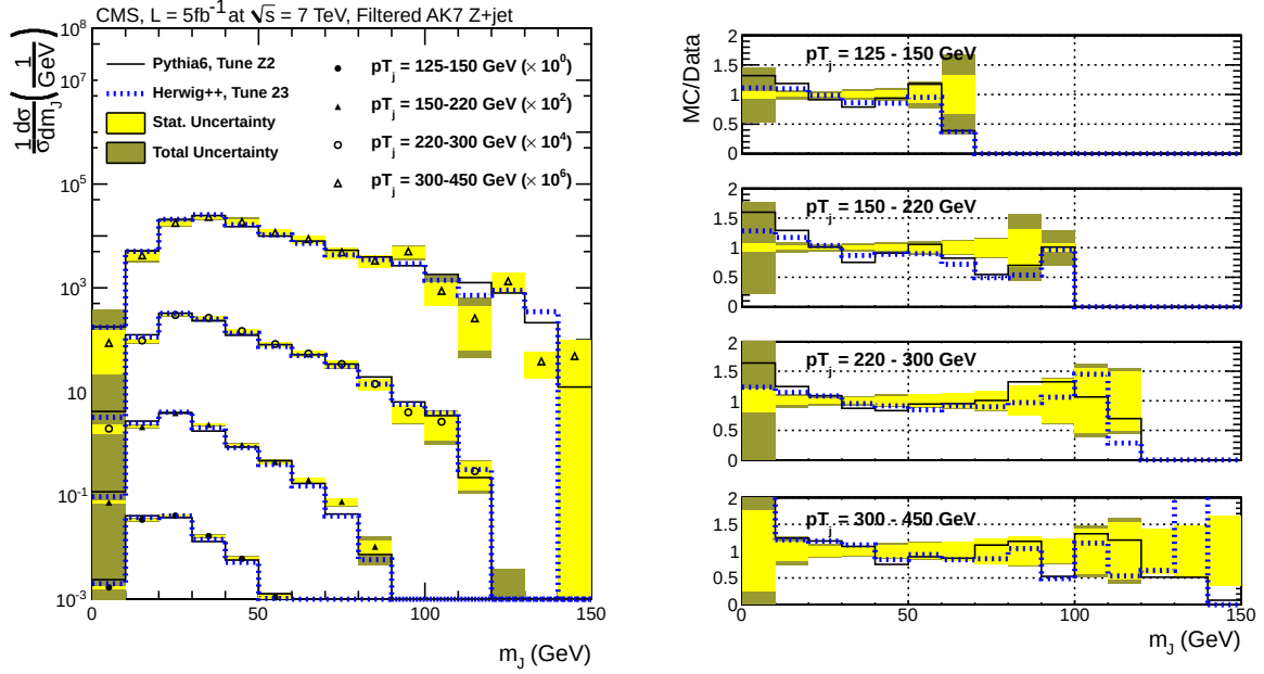
Figure 13: Unfolded AK7 filtered m_j distribution for Z(\ell\ell)+\text{jet} events. The data (black symbols) are compared to MC expectations from MADGRAPH+PYTHIA6 (solid lines) and HERWIG++ (dotted lines) on the left. The ratio of MC to data is given on the right. The statistical uncertainty is shown in light shading, and the total uncertainty in dark shading.
