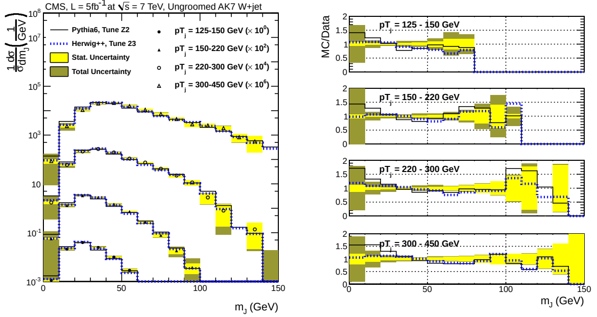
Figure 18: Distributions in m_J for unfolded, ungroomed AK7 jets in W(\ell\nu_\ell)+\text{jet} events. The data (black symbols) are compared to MC expectations from MADGRAPH+PYTHIA6 (solid lines) and HERWIG++ (dotted lines) on the left. The ratios of MC to data are given on the right. The statistical uncertainty is shown in light shading, and the total uncertainty in dark shading.
