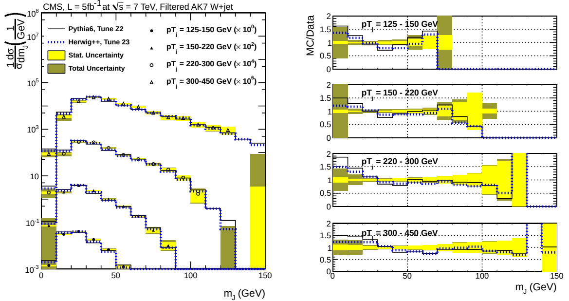
Figure 19: Distributions in m_J for unfolded, filtered AK7 jets in W(\ell\nu_\ell)+\text{jet} events. The data (black symbols) for different bins in p_T are compared to MC expectations from MADGRAPH+PYTHIA6 (solid lines) and HERWIG++ (dotted lines) on the left. The ratios of MC to data are given on the right. The statistical uncertainty is shown in light shading, and the total uncertainty in dark shading.
