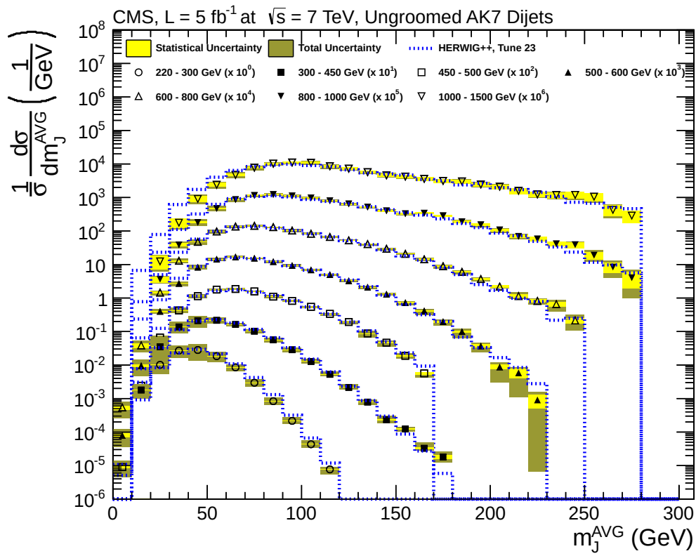
Figure 4: Unfolded distributions for the mean mass of the two leading jets in dijet events for reconstructed AK7 jets, separated according to intervals in p_T^{\text{AVG}} (the mean p_T of the two jets). The data are shown by the symbols indicating different bins in the mean p_T of the two jets. The statistical uncertainty is shown in light shading, and the total uncertainty in dark shading. Predictions from HERWIG++ are given by the dotted lines. To enhance visibility, the distributions for larger values of p_T^{\text{AVG}} are scaled up by the factors given in the legend.
