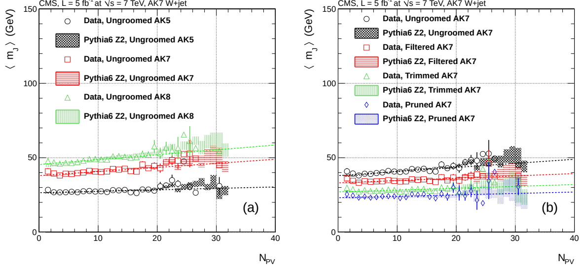
Figure 3: Distributions of the average jet mass for AK jets as a function of the number of reconstructed primary vertices: (a) for different jet radii, and (b) for AK7 jets, comparing the impact of grooming algorithms to results without grooming.
