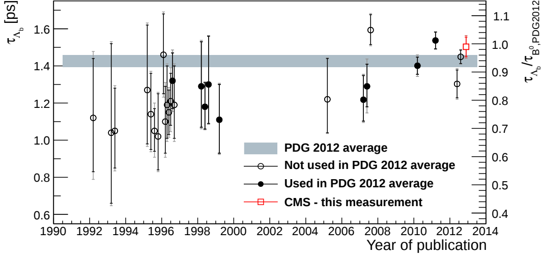
Figure 4: Evolution over time of the \Lambda_b^0 lifetime measurements (left scale) [9–28] and the ratio of the measurements to the 2012 world-average B^0 lifetime \tau_{B^0} [32] (right scale). The values shown as open circles were not included in the Particle Data Group (PDG) 2012 average [32], displayed as the grey band, while those shown as filled circles were included. The result of this analysis is shown by the open square. The inner error bars represent the statistical uncertainties, and the outer error bars show the combined statistical and systematic uncertainties added in quadrature. Where needed, points have been shifted slightly along the time axis to enhance clarity.
