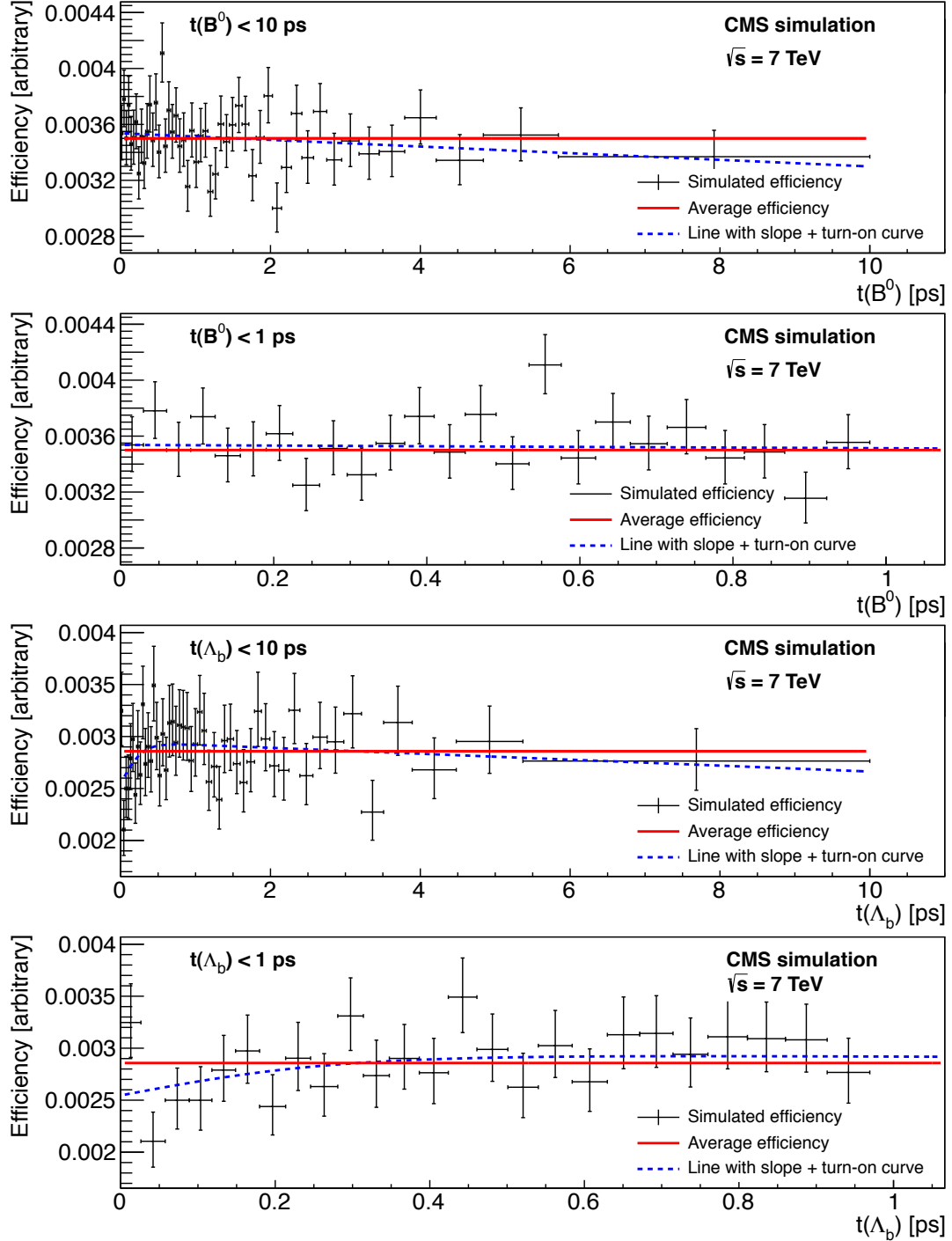
Figure 1: The overall reconstruction and selection efficiency (in arbitrary units) as a function of proper decay time for B^0 (upper two plots) and \Lambda_b^0 (lower two plots). The second and fourth plots show the B^0 and \Lambda_b^0 efficiencies, respectively, for smaller proper decay times t < 1 ps. The horizontal solid lines show the average efficiency, while the dashed lines display the result of the fits to the function given by Eq. (2).
